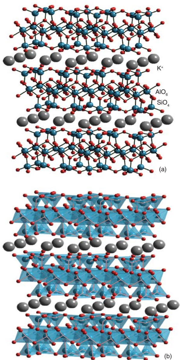
Figure 14.18 (a)* The structure of 2:1 clay minerals such as muscovite mica \text{KAl}_2(\text{OH})_2\text{Si}_3\text{AlO}_{10} , in which \text{K}^+ resides between the charged layers (exchangeable cation sites), \text{Si}^{4+} resides in sites of coordination number 4, and \text{Al}^{3+} in sites of coordination number 6; (b)* the polyhedral representation. In talc, \text{Mg}^{2+} ions occupy the octahedral sites and O atoms on the top and bottom are replaced by OH groups and the \text{K}^+ sites are vacant.
