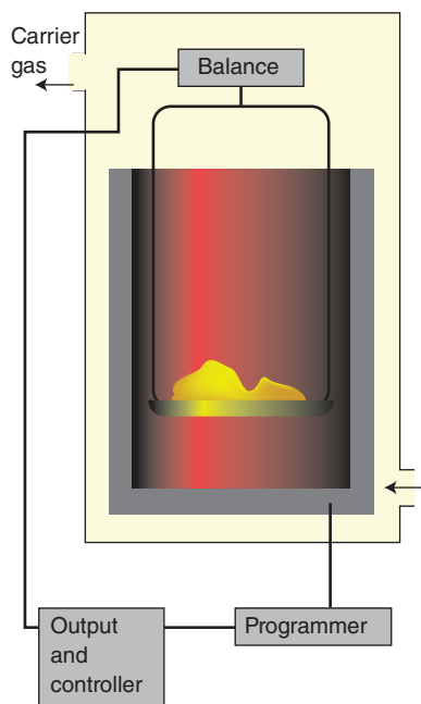
Figure 8.47 A thermogravimetric analyser: the mass of the sample is monitored as the temperature is raised.
