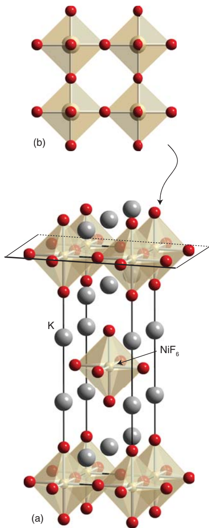
Figure 24.21* The K 2 NiF 4 structure: (a) the displaced layers of NiF 6 octahedra interspersed with K + ions, and (b) a view of one layer of composition NiF 4 showing the corner-sharing octahedra linked through F.
