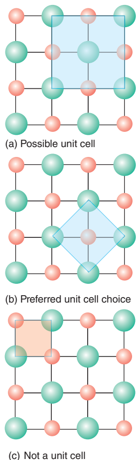
Figure 3.1 A two-dimensional solid and two choices of a unit cell. The entire crystal is produced by translational displacements of either unit cell, but (b) is generally preferred to (a) because it is smaller.
