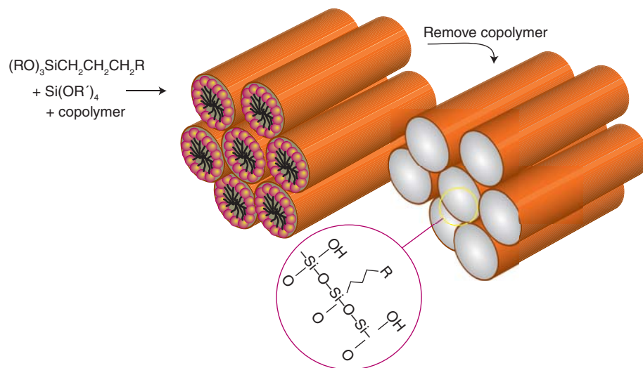
Figure 24.90 Block-copolymer structure-directing agents self-assemble into micellar rods forming hexagonal arrays that can be removed to yield nanoporous silica matrices for inclusion chemistry and catalysis. (Adapted from M.E. Davis, Chem. Rev. , 2002, 102 , 3601.)
