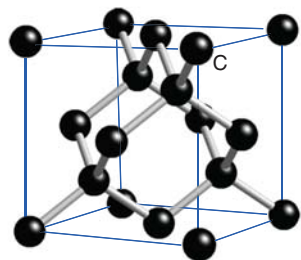
Figure 14.1* The cubic diamond structure.
