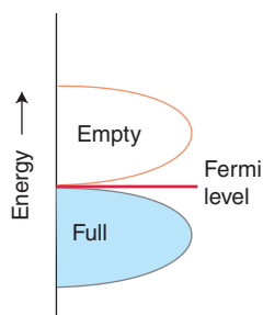
Figure 3.70 The density of states in a semimetal.
