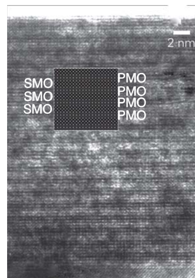
Figure 24.88 Cross-sectional TEM image of a 2 \times 2 superlattice of SrMnO_3 and PrMnO_3 prepared using laser-MBE. The inset shows a calculated image confirming the (SrMnO_3)_2(PrMnO_3)_2 structure. (From B. Mercey, et al., In situ monitoring of the growth and characterization of (PrMnO_3)_n(SrMnO_3)_n superlattices. J. Appl. Phys. , 2003, 94 , 2716; reprinted with permission from the American Institute of Physics.)
