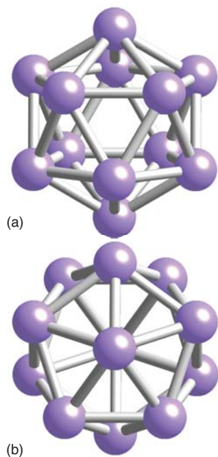
Figure 13.1 A view of the B_{12} icosahedron in rhombohedral boron (a) along and (b) perpendicular to the three-fold axis of the crystal. The individual icosahedra are linked by 3c,2e bonds.
