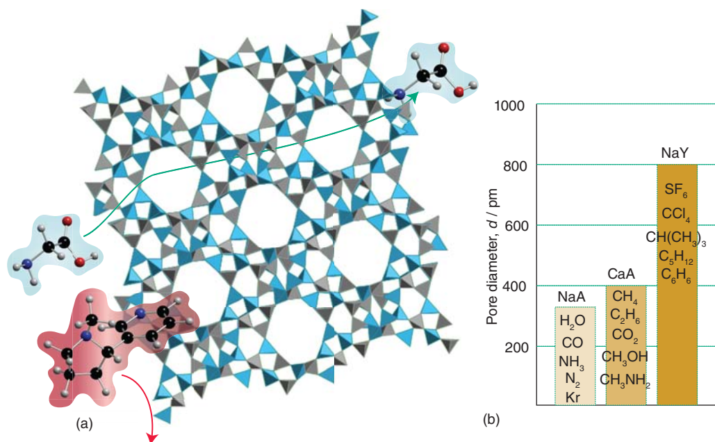
Figure 24.48* The use of porous zeolite structures for the separation of molecules of various sizes. (a) Only the smaller molecule can diffuse into and then out of the zeolite pore, so a membrane of this material may be used to separate this mixture. (b) The maximum molecular size that can be absorbed into various zeolite channel diameters. NaY is faujasite, a moderately large pore zeolite.
