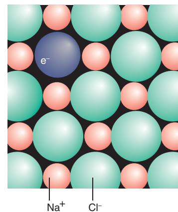
Figure 3.57 An F-centre is an electron that occupies an anion vacancy. The energy levels of the electron resemble those of a particle in a three-dimensional square well.
