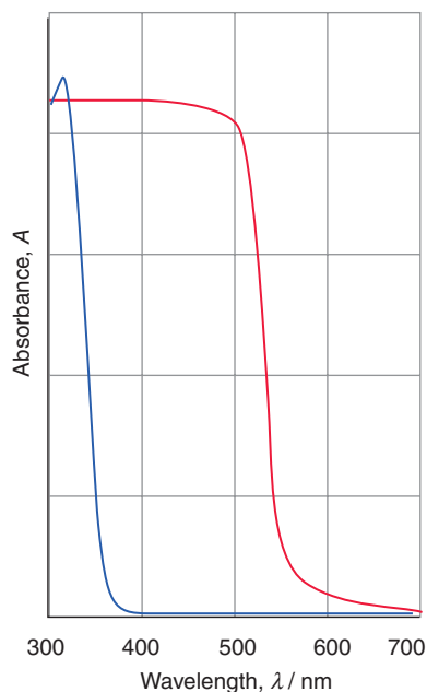
Figure 8.13 The UV-visible spectra of \text{PbCrO}_4 (red) and \text{TiO}_2 (blue). Absorbance is given as a function of wavelength.
