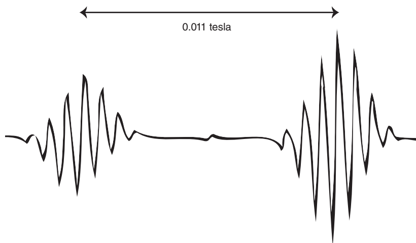
Figure 23.17 The EPR spectrum of \text{Pu}^{3+} doped into \text{CaF}_2 , showing the doublet due to hyperfine coupling with ^{239}\text{Pu} ( I = \frac{1}{2} ) and the superhyperfine coupling with eight equivalent \text{F}^- ( I = \frac{1}{2} ).
