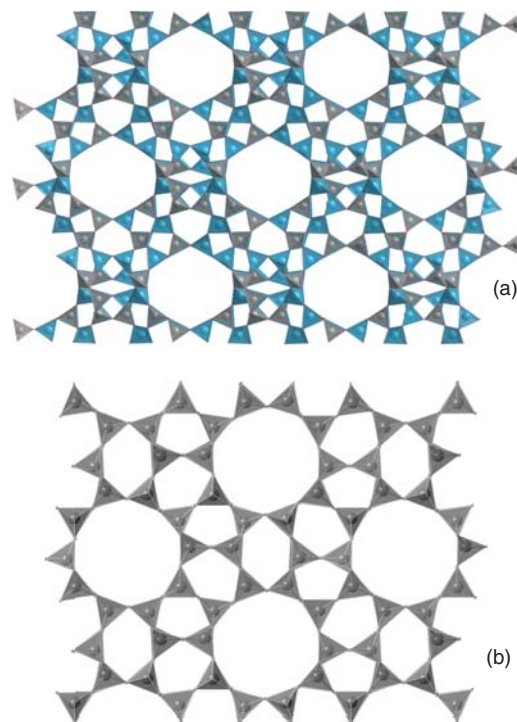
Figure 14.20 Two zeolite framework structures: (a)* Zeolite-X and (b)* ZSM-5. In each case just the \text{SiO}_4 tetrahedra that form the framework are shown; nonframework atoms such as charge-balancing cations and water molecules are omitted.
