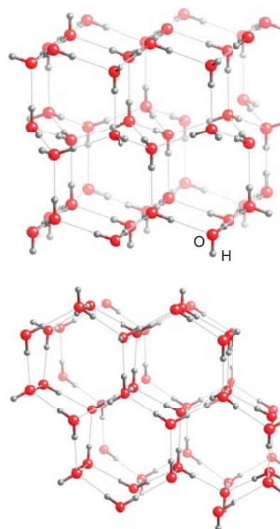
Figure 10.7* The structure of the hexagonal form of ice ( \text{I}_h ) shown in two orientations.
