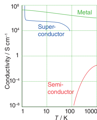
Figure 3.60 The variation of the electrical conductivity of a substance with temperature is the basis of the classification of the substance as a metallic conductor, a semiconductor, or a superconductor.
