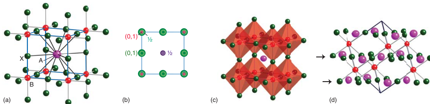
Figure 3.42 The perovskite structure, ABX_3 : (a) the cubic unit cell outlined in blue, emphasizing the coordination geometry of the A (12-fold) and B (6-fold octahedral) cations to X; (b) the projection representation of the unit cell; (c)* the same structure, emphasizing the octahedral coordination of the B sites and description of the structure as linked BX_6 octahedra; (d) the relationship of the perovskite structure to a close-packed arrangement of A and X (arrowed) with B in octahedral holes; the unit cell outlined is the same as that in (a).
