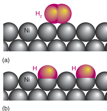
Figure 25.16 Schematic representation of (a) physisorption and (b) chemisorption of hydrogen on a nickel metal surface.
