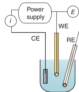
Figure 8.51 An electrochemical cell into which three electrodes are placed. The half-cell reaction of interest occurs at the working electrode (WE), the potential of which is controlled with respect to the reference electrode (RE). No current flows between the WE and the RE: current flows instead between the WE and the counter electrode (CE) at which reactions such as solvent or electrolyte breakdown are driven in order to balance the charge passed across the WE.
