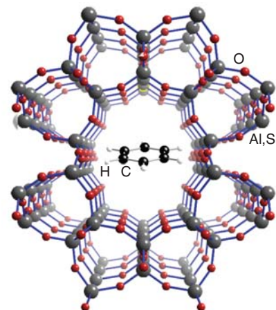
Figure 25.15* A view into the channels of zeolite theta-1 with an adsorbed benzene molecule in the large central channel. (Based on A. Dyer, An introduction to molecular sieves . John Wiley & Sons (1988).)
