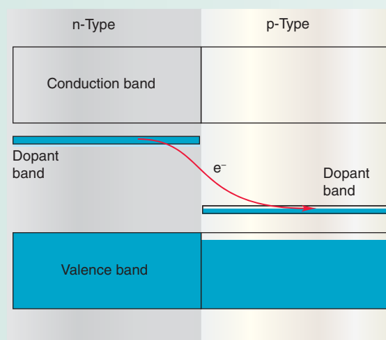
Figure B24.3 The structure of a p–n junction.
