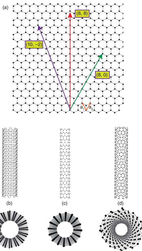
Figure 24.80 (a) The honeycomb structure of a graphene sheet. Single-walled carbon nanotubes can be formed by folding the sheet along lattice vectors, two of which are shown as a_1 and a_2 . Folding along the (8,8) , (8,0) , and (10,-2) vectors leads to armchair (b), zigzag (c), and chiral (d) tubes, respectively. (Based on H. Dai, Acc. Chem. Res. , 2002, 35 , 1035; reproduced with permission from the American Chemical Society.).
