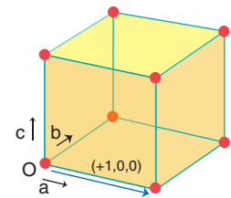
Figure 3.3 Lattice points describing the translational symmetry of a primitive cubic unit cell. The translational symmetry is just that of the unit cell; for example the a lattice point at the origin, O, translates by (+1,0,0) to another corner of the unit cell.
