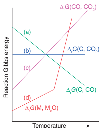
Figure 5.15 Part of an Ellingham diagram showing the standard Gibbs energy for the formation of a metal oxide and the three carbon oxidation Gibbs energies. The slopes of the lines are determined largely by whether there is net gas formation or consumption in the reaction. A phase change generally results in a kink in the graph (because the entropy of the substance changes).
