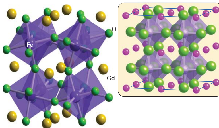
Figure 23.11* The \text{GdFeO}_3 structure type, with the \text{FeO}_6 octahedra outlined. Inset shows how the \text{GdFeO}_3 structure is related to the perovskite structure.
