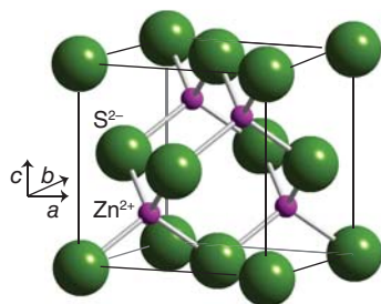
Figure 3.6* The cubic ZnS structure.
