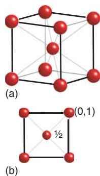
Figure 3.22 (a)* A bcc structure unit cell and (b) its projection representation.
