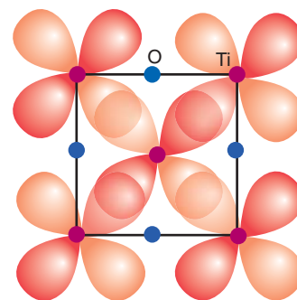
Figure 3.66 One face of the TiO rock-salt structure showing how orbital overlap can occur for the d_{xy} , d_{yz} , and d_{zx} orbitals.
