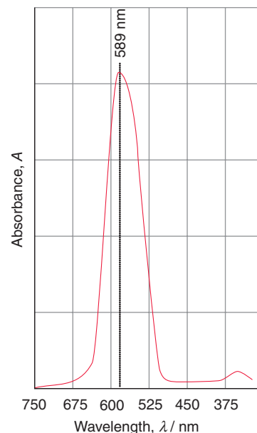
Figure 8.11 The UV-visible absorption spectrum of the solid ultramarine blue, \text{Na}_7[\text{SiAlO}_4]_6(\text{S}_3) .
