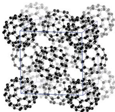
Figure 24.68* The arrangement of C_{60} molecules in a face-centred cubic lattice in the crystalline material.
