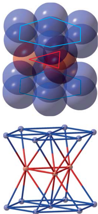
Figure 3.13* The hexagonal close-packed (hcp) unit cell of the ABAB... polytype. The colours of the spheres correspond to the layers in Fig. 3.12c.
