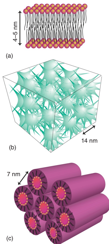
Figure 24.91 Representations of three types of ordered mesoporous solids: (a) hexagonal lamellar (layered materials), (b) cubic (complex arrangements), and (c) hexagonal (honeycomb). (Adapted from A. Mueller and D.F. O'Brien, Chem. Rev. , 2002, 102, 729.)
