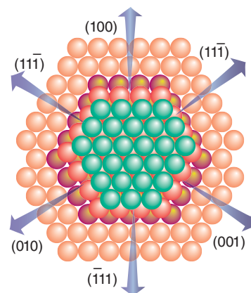
Figure 25.18 Some possible metal crystal planes that might be exposed on a metal surface to a reactive gas. The planes labelled [\bar{1} \ 1 \ 1] , [1 \ \bar{1} \ 1] , etc. are hexagonally close-packed and the planes represented by [100] , [010] , etc. have square arrays of atoms.
