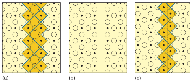
Figure 24.2 The concept of a crystallographic shear plane, illustrated by the (100) plane of the \text{ReO}_3 structure. (a) A plane of metal (Re) and oxygen (O) atoms. The octahedron around each metal atom is completed by a plane of oxygen atoms above and below the plane illustrated here. Some of the octahedra are shaded to clarify the processes that follow. (b) Oxygen atoms in the plane perpendicular to the page are removed, leaving two planes of metal atoms that lack their sixth oxygen ligand. (c) The octahedral coordination of the two planes of metal atoms is restored by translating the right slab as shown. This creates a plane (labelled a shear plane), vertical to the page, in which the \text{MO}_6 octahedra share edges.
