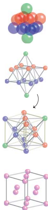
Figure 3.14 The cubic close-packed (fcc) unit cell of the ABC... polytype. The colours of the spheres correspond to the layers in Fig. 3.12d.
