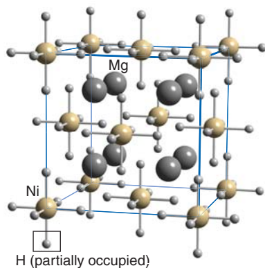
Figure 24.62* The idealized structure of cubic \text{Mg}_2\text{NiH}_4 ; hydrogen sites are only partially occupied.
