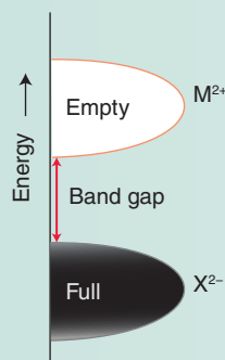
Figure B19.7 The simple band structure of \text{MX} salts.
