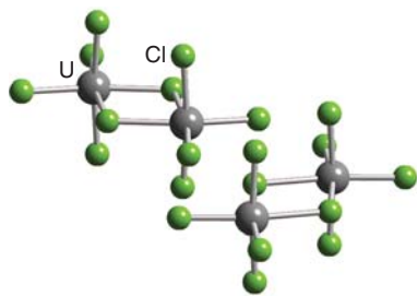
Figure 23.19* The crystal structure of \text{U}_2\text{Cl}_{10} consists of discrete molecules formed from pairs of edge-sharing \text{UCl}_6 octahedra.
