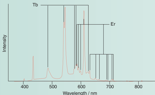
Figure B23.1 Spectrum of a fluorescent lamp, showing lines arising from lanthanoid ions in the phosphor.
