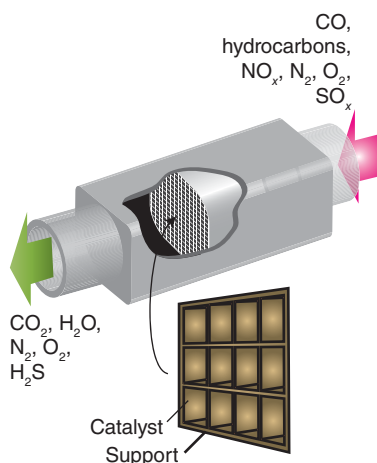
Figure 25.4 A heterogeneous catalyst in action. The automobile catalytic converter oxidizes CO and hydrocarbons, and reduces nitrogen and sulfur oxides. The particles of a metal catalyst are supported on a robust ceramic honeycomb.
