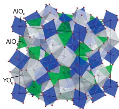
Figure 19.2* Yttrium aluminium garnet, YAG, \text{Y}_3\text{Al}_5\text{O}_{12} .
