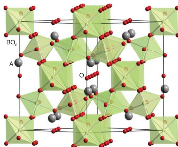
Figure 24.26* The pyrochlore structure adopted by many compounds of stoichiometry A_2B_2O_7 . The BO_6 octahedra are shown, and form channels containing the A-type cations and oxide ions.
