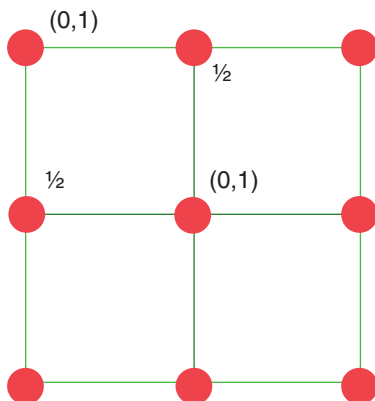
Figure 3.9 The projection representation of an fcc unit cell.
