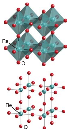
Figure 24.16* The \text{ReO}_3 structure shown as the unit cell, and the \text{ReO}_6 octahedra forming the unit cell.
