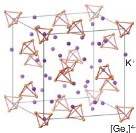
Figure 3.28* The structure of the Zintl phase KGe showing the [\text{Ge}_4]^{4-} tetrahedral units and interspersed \text{K}^+ ions.
