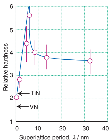
Figure 24.86 The dependence of hardness on the superlattice period for (\text{TiN})_m(\text{VN})_m superlattices. (Adapted from U. Helmerson, et al., J. Appl. Phys. , 1987, 62 , 481.)
