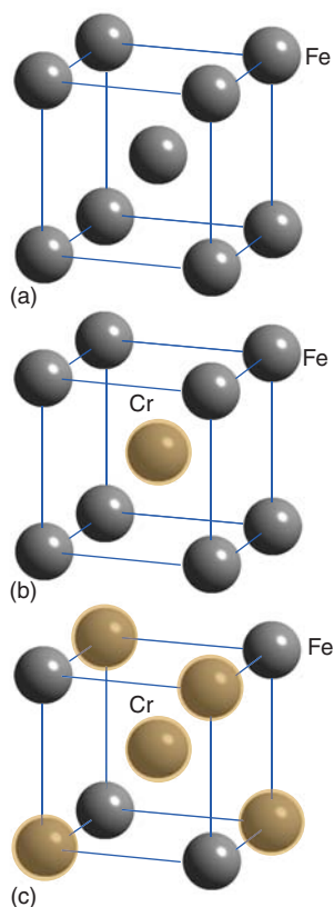
Figure 3.29* The structures of (a) iron, (b) FeCr, and (c) a Fe/Cr alloy (see Selftest 3.8 ).
