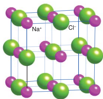
Figure 11.4* The rock-salt structure adopted by the majority of Group 1 metal halides.
