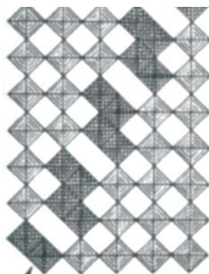
Figure 24.3 (a) High-resolution electron micrograph lattice image of a crystallographic shear plane in \text{WO}_{3-x} . (b) The oxygen octahedral polyhedra that surround the W atoms imaged in the electron micrograph; note the edge-shared octahedra along the crystallographic shear plane. (Reproduced by permission from S. Iijima, J. Solid State Chem. 1975, 14, 52.)
