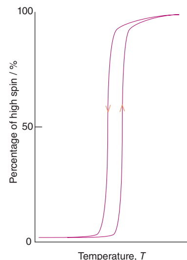
Figure 20.44 A hysteresis loop that can occur with some spin-crossover systems.
