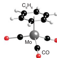
12 [\text{Mo}(\eta^6\text{-C}_6\text{H}_6)(\text{CO})_3]
