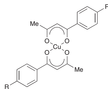
7 \beta -diketone complex
