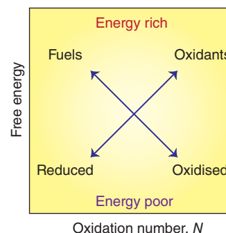
Figure 5.19 A generic Frost diagram depicting the relationships between fuels, oxidants, and energy-poor compounds such as water, carbon dioxide, and ash.
