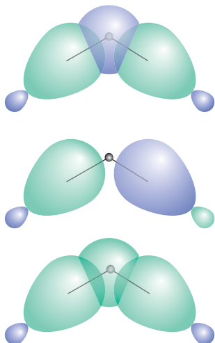
Figure 2.34 The molecular orbital formed between two B atoms and one H atom lying between them, as in \text{B}_2\text{H}_6 . Two electrons occupy the bonding combination and hold all three atoms together.
