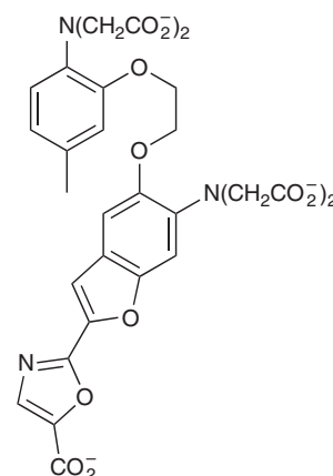
13 FURA-2, a fluorescent ligand for \text{Ca}^{2+}
