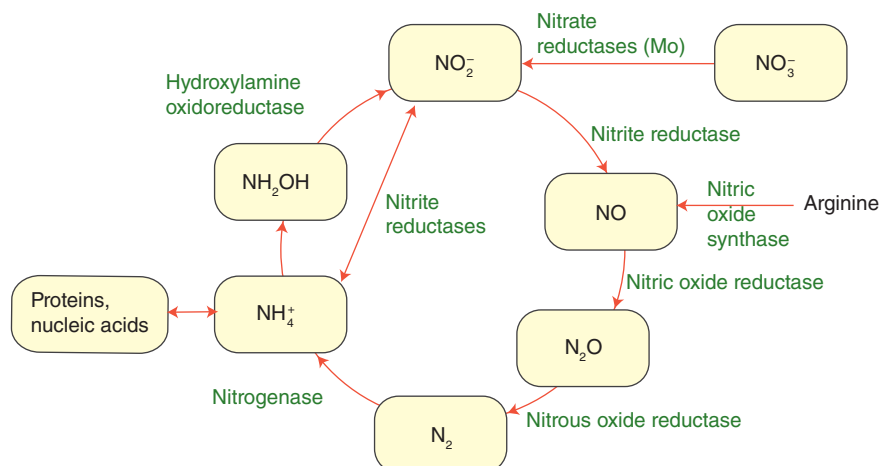
Figure 26.48 The biological nitrogen cycle showing the enzymes involved.
