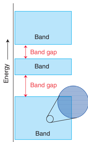
Figure 3.61 The electronic structure of a solid is characterized by a series of bands of orbitals separated by gaps at energies where orbitals do not occur.
