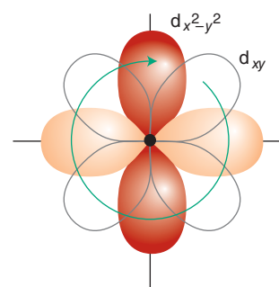
Figure 20.6* If there is a low-lying orbital of the correct symmetry, the applied field may induce the circulation of the electrons in a complex and hence generate orbital angular momentum. This diagram shows the way in which circulation may arise when the field is applied perpendicular to the xy -plane (perpendicular to this page).
