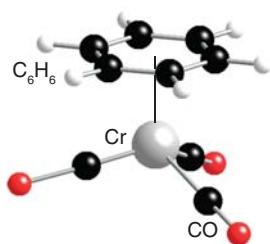
79 [\text{Cr}(\eta^6\text{-C}_6\text{H}_6)(\text{CO})_3]
