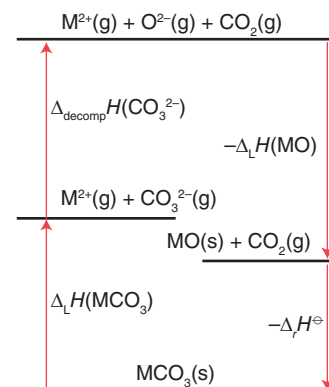
Figure 3.49 A thermodynamic cycle showing the enthalpy changes involved in the decomposition of a solid carbonate MCO 3 .
