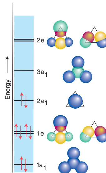
Figure 2.29 A schematic illustration of the molecular orbitals of \text{NH}_3 with the size of the atomic orbital indicating the magnitude of its contribution to the molecular orbital. The view is along the z -axis.
