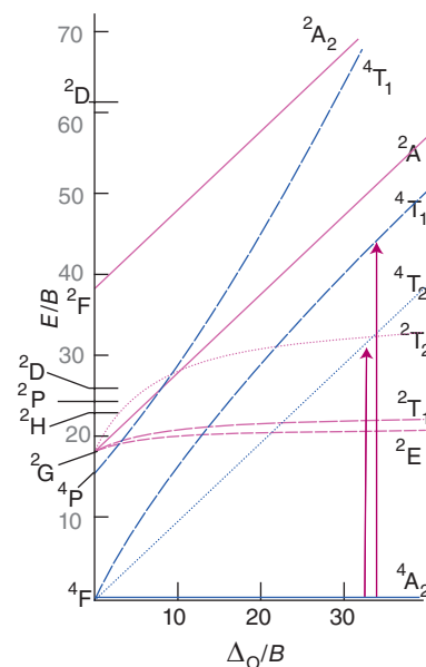
Figure 20.31 The Tanabe–Sugano diagram for the d^3 configuration. Note that the left-hand axis corresponds to Fig. 20.24 (right). A complete collection of diagrams for d^n configurations is given in Resource section 6. The parity subscript g has been omitted from the term symbols for clarity.
