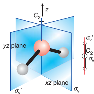
Figure 6.10* The symmetry elements of H_2O . The diagram on the right is the view from above and summarizes the diagram on the left.
