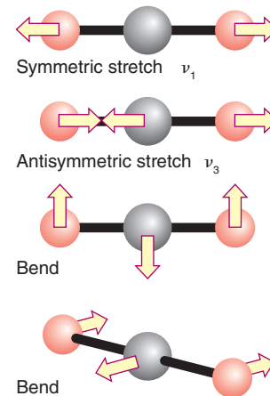
Figure 6.16* The stretches and bends of a \text{CO}_2 molecule.
