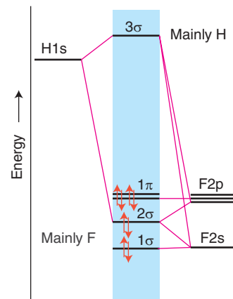
Figure 2.21* The molecular orbital energy-level diagram for HF. The relative positions of the atomic orbitals reflect the ionization energies of the atoms.
