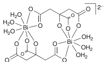
18 [\text{Bi}_2(\text{cit})_2]^{2-}
