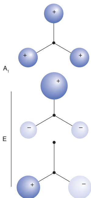
Figure 6.21* The (a) A 1 and (b) E symmetry-adapted linear combinations of H1s orbitals in NH 3 .
