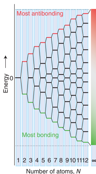
Figure 3.63 The energies of the orbitals that are formed when N atoms are brought up to form a one-dimensional array. This produces a density-of-states diagram similar to that shown in Fig. 3.68.
