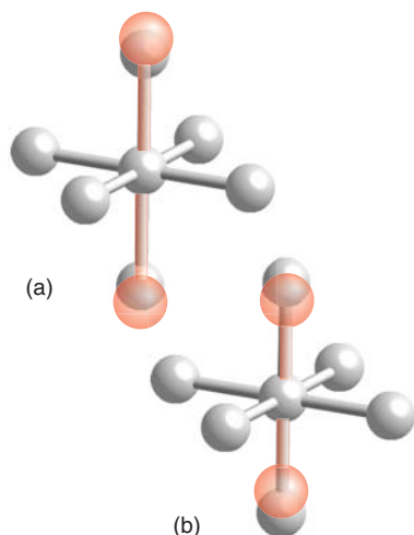
Figure 20.11* (a) A tetragonally distorted complex where two of the ligands have moved further away from the central ion. (b) A tetragonally distorted complex where two of the ligands have moved closer towards the central ion.
