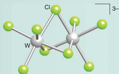
B7 [\text{Cl}_3\text{W}(\mu\text{-Cl})_3\text{WCl}_3]^{3-}
