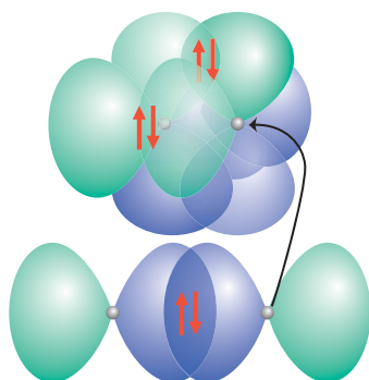
Figure 2.5 The VB description of N_2 . Two electrons form a \sigma bond and another two pairs form two \pi bonds. In linear molecules, where the x - and y -axes are not specified, the electron density of \pi bonds is cylindrically symmetrical around the internuclear axis.
