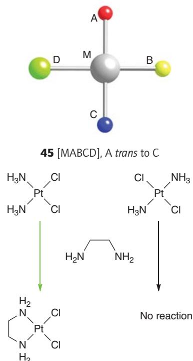
Figure 7.4 The preparation of cis - and trans -diamminedichloroplatinum(II) and a chemical method for distinguishing the isomers.
