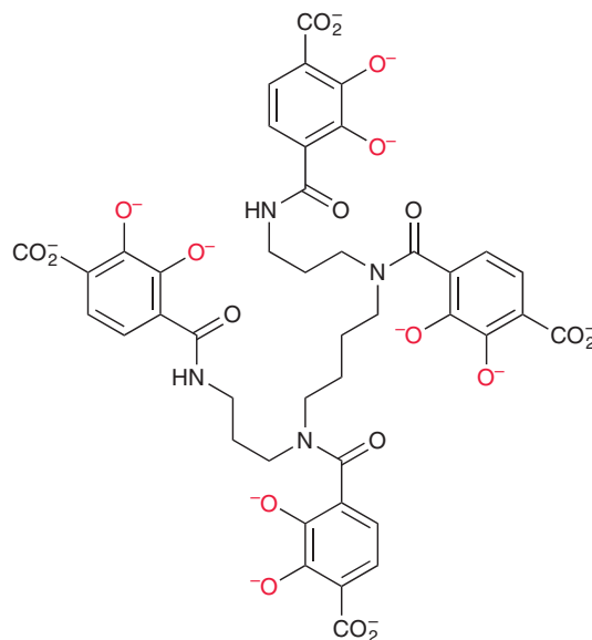
17 Enterobactin
