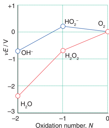
Figure 5.7 The Frost diagram for oxygen in acidic solution (red line, \text{pH}=0 ) and alkaline solution (blue line, \text{pH}=14 ).
