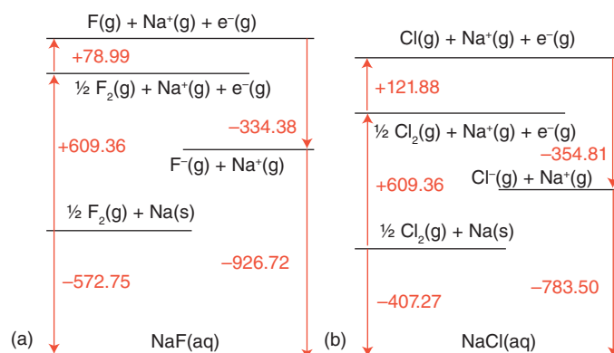
Figure 17.10 Thermochemical cycles for the enthalpy of formation of (a) aqueous sodium fluoride and (b) aqueous sodium chloride. The hydration is much more exothermic for F^- than for Cl^- . All values are in \text{kJ mol}^{-1} .
