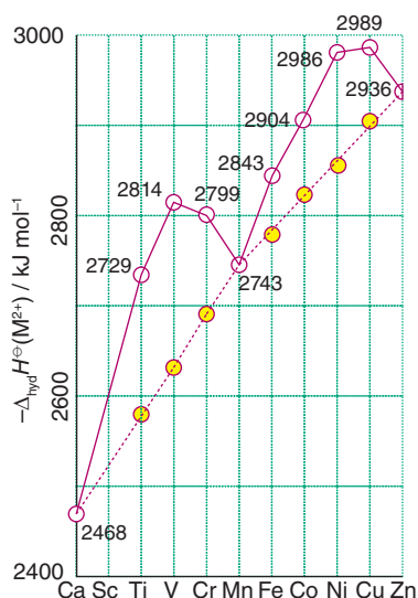
Figure 20.7 The hydration enthalpy of M^{2+} ions of the first row of the d block. The straight dotted lines show the trend when the ligand-field stabilization energy has been subtracted from the observed values. Note the general trend to greater hydration enthalpy (more exothermic hydration) on crossing the period from left to right.
