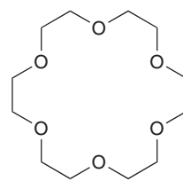
1 18-crown-6
