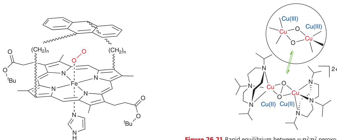
22 'Basket' Fe-porphyrin with O_2 bound
