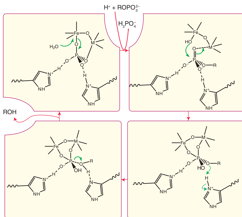
Figure 26.33 Proposed mechanism of action of acid phosphatase. The metal site M(II) is occupied by Fe (most common in animals) or by Mn or Zn (in plants).
