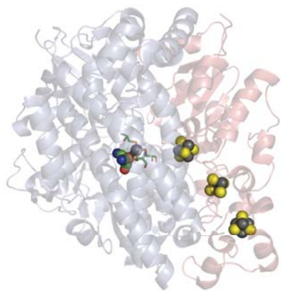
Figure 26.27* A series of three Fe–S clusters provides a long-range electron transfer pathway to the buried active site in hydrogenases.
