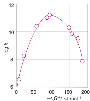
Figure 21.21 Plot of \log_{10} k against -\Delta_r G^\ominus for the iridium complex (20) in acetonitrile solution at room temperature, the free energy of reaction is varied by use of different R groups on the rigid complex.
