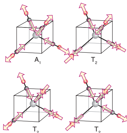
Figure 6.19* The modes of [\text{Ni}(\text{CO})_4] that correspond to the stretching of CO bonds.
