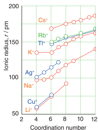
Figure 3.45 The variation of ionic radius with coordination number.
