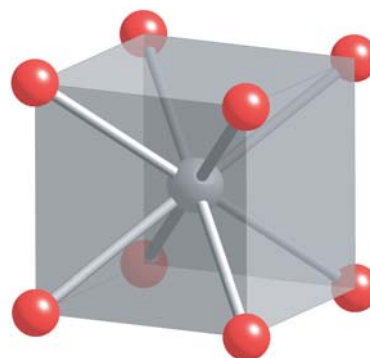
30 Cube
