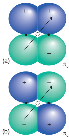
Figure 2.16 (a) Bonding and (b) antibonding \pi interactions, with the arrow indicating the inversions.
