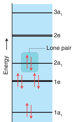
Figure 6.25 A schematic molecular orbital energy-level diagram for \text{NH}_3 and an indication of its ground-state electron configuration.
