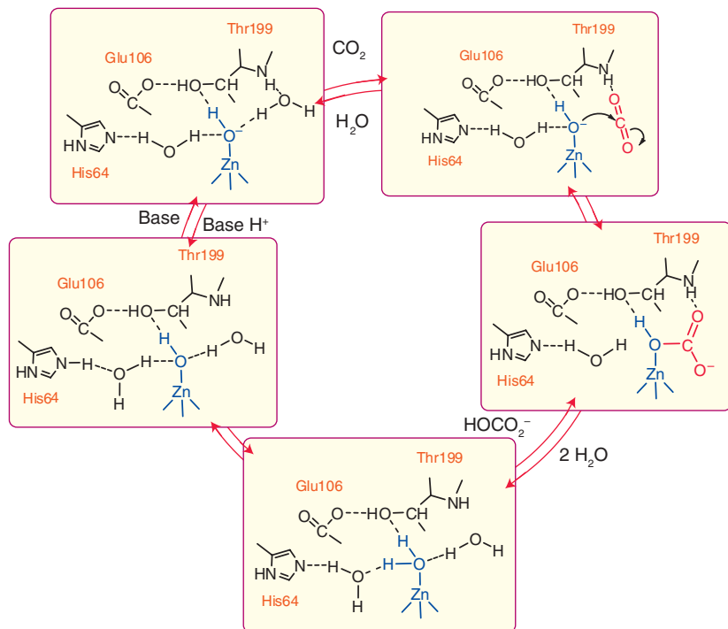
Figure 26.30 The mechanism of action of carbonic anhydrase, indicating the importance of proton transfer pathways in this very fast reaction.
