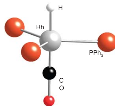
9 [\text{Rh}(\text{CO})\text{H}(\text{PPh}_3)_3]
