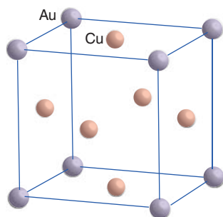
Figure 3.75* The structure of \text{Cu}_3\text{Au} .
