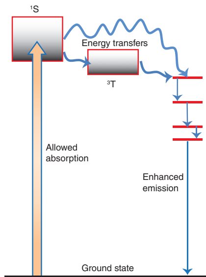
Figure 23.8 A Jablonski diagram represents the processes by which energy is transferred from a light-absorbing antenna to the emission levels of a luminescent centre.
