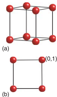
Figure 3.23 (a)* A primitive cubic unit cell and (b) its projection representation.
