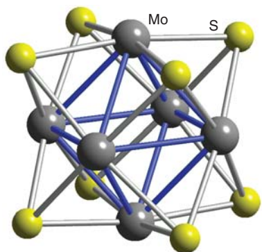
Figure 24.43* The \text{Mo}_6\text{S}_8 unit present in a Chevrel-phase \text{Pb}_x\text{Mo}_6\text{S}_8 .
