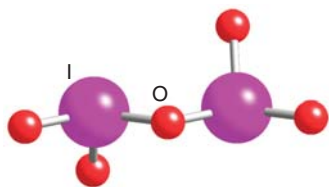
15 \text{I}_2\text{O}_5
