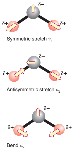
Figure 6.15* The vibrations of an \text{H}_2\text{O} molecule all change the dipole moment.
