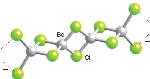
1 (\text{BeCl}_2)_n
