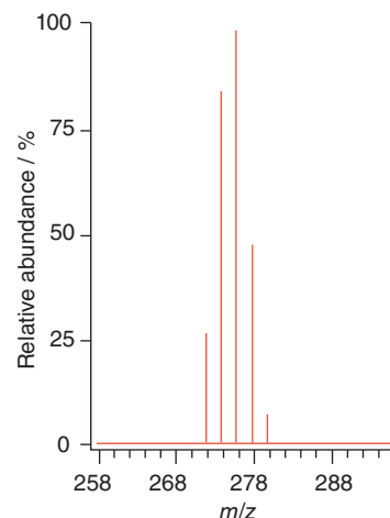
Figure 8.42 The mass spectrum of a sample containing mercury, showing the isotopic composition of the atoms.
