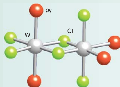
B6 [(\text{py})_2\text{Cl}_2\text{W}(\mu\text{-Cl})_2\text{WCl}_2(\text{py})_2]
