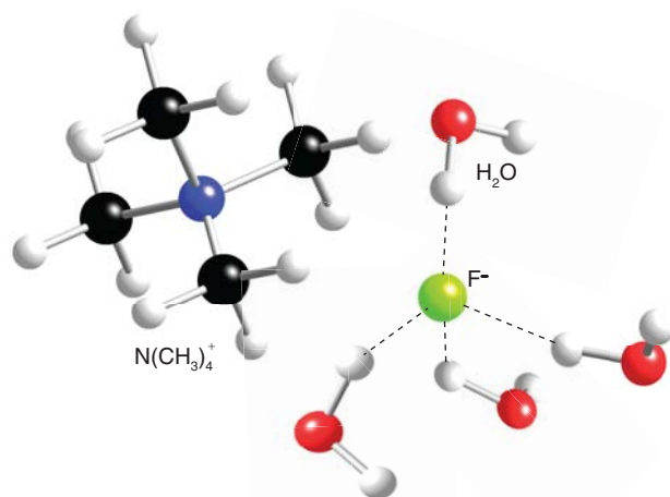
6 \text{N}(\text{CH}_3)_4\text{F}\cdot 4\text{H}_2\text{O}
