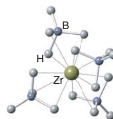
1 [\text{Zr}(\text{BH}_4)_4]
