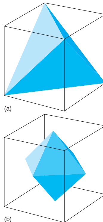
Figure 6.11* Shapes having cubic symmetry: (a) the tetrahedron, point group T_d ; (b) the octahedron, point group O_h .
