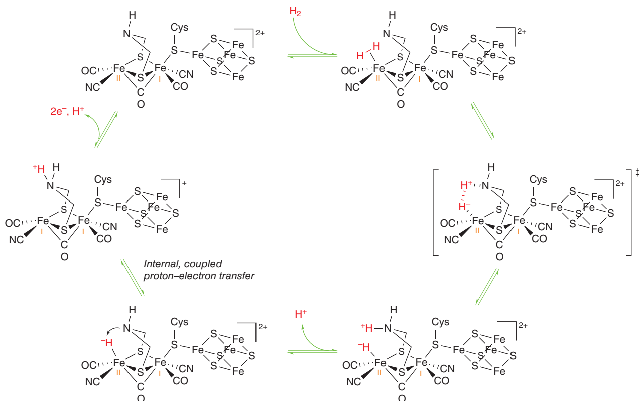
Figure 26.50 Proposed catalytic cycle of hydrogenase.
