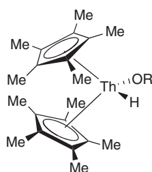
5 [\text{Th}(\text{Cp}^*)(\text{H})(\text{OR})]
