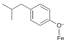
7 Fe-tyrosine coordination
