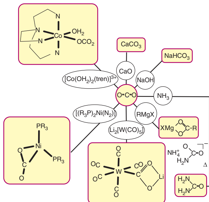
Figure 14.11 Characteristic reactions of carbon dioxide.
