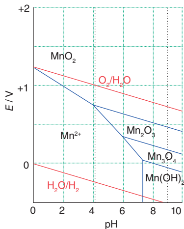
Figure 5.13 A section of the Pourbaix diagram for manganese. The broken black vertical lines represent the normal pH range in natural waters.
