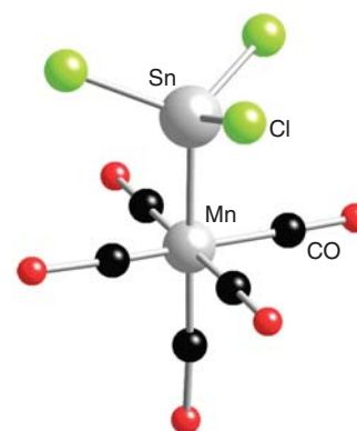
19 [\text{Mn}(\text{CO})_5(\text{SnCl}_3)]
