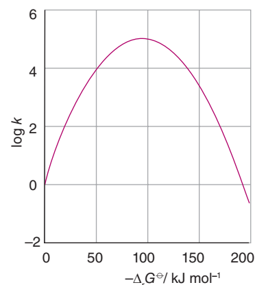
Figure 21.20 The theoretical dependence of the \log_{10} of the reaction rate (in arbitrary units) on \Delta_r G^\ominus for a redox reaction with \lambda = 1.0 \text{ eV} ( 100 \text{ kJ mol}^{-1} ).
