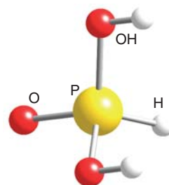
7 \text{OPH}(\text{OH})_2 , \text{H}_3\text{PO}_3
