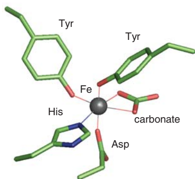
19* An Fe-binding site in transferrin
