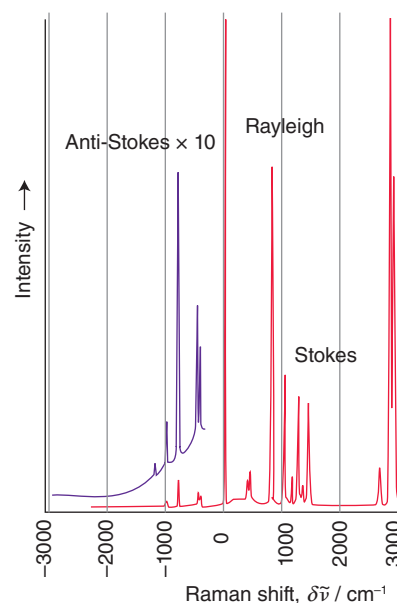
Figure 8.21 A typical Raman spectrum showing Rayleigh scattering (scattering of the laser light with no change in wavelength that occurs at the origin) and Stokes and anti-Stokes lines.
