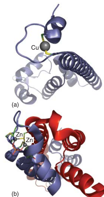
Figure 26.56 Comparison of the (a)* Cu-binding and (b)* Zn-binding sites in the respective transcription factors CueR and ZntR. Note how Cu(I) is recognized by a linear binding site (to two cysteines) whereas Zn is recognized by an arrangement of Cys and His ligands that binds two Zn(II) atoms together with a bridging phosphate group.
