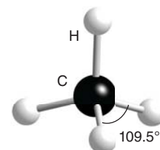
1 Methane, \text{CH}_4
