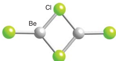
3 (\text{BeCl}_2)_2
