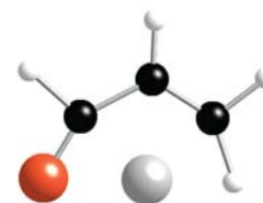
49 anti
