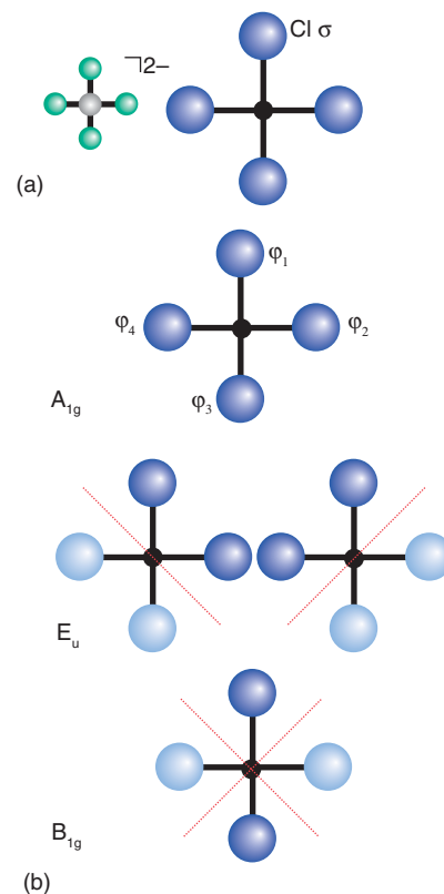
Figure 6.28 (a) The Cl orbital basis used to construct SALCs in [\text{PtCl}_4]^{2-} , and (b) the SALCs constructed for [\text{PtCl}_4]^{2-} .
