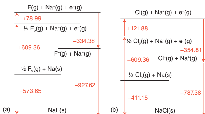
Figure 17.1 Thermochemical cycles for (a) sodium fluoride and (b) sodium chloride. All values are in kJ mol -1 .
