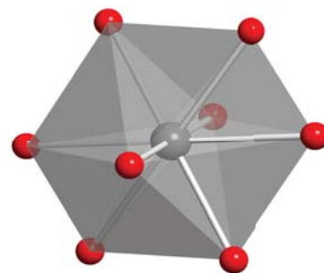
27 Dodecahedron D_{2d}
