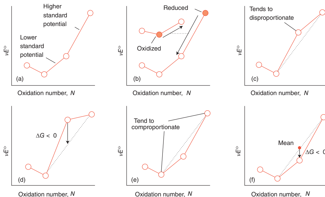
Figure 5.9 The interpretation of a Frost diagram to gauge (a) reduction potential; (b) tendency towards oxidation and reduction; (c), (d) disproportionation; (e), (f) comproportionation.
