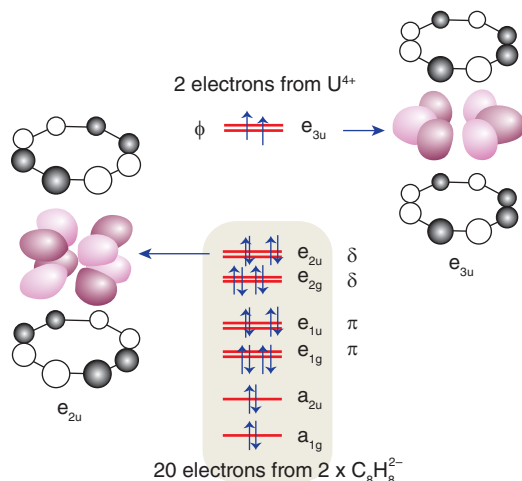
Figure 23.20 Partial molecular orbital diagram for actinoid \eta^8 -cyclooctatetraene sandwich complexes, showing how the 6d and 5f atomic orbitals interact with the C p_x orbitals (only one lobe is shown).
