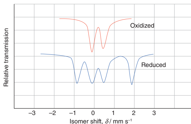
Figure 26.60 Mössbauer spectra of a sample of ferredoxin from chloroplasts at 77 K.
