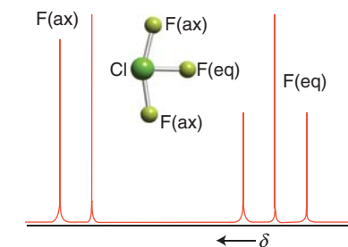
Figure 8.26 The ^{19}\text{F} -NMR spectrum of \text{ClF}_3 .
