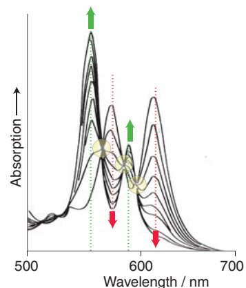
Figure 8.16 Isosbestic points (circled) observed in the absorption spectral changes during reaction of \text{HgTPP} ( \text{TPP} =tetraphenylporphyrin) with \text{Zn}^{2+} in which \text{Zn} replaces \text{Hg} in the macrocycle. The initial and final spectra are those of the reactant and product, which indicates that the \text{TPP} does not reach a detectable concentration during the reaction. Adapted from C. Grant and P. Hambright, J. Am. Chem. Soc. , 1969, 91 , 4195.
