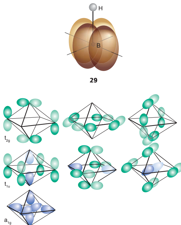
Figure 13.9 Radial and tangential bonding molecular orbitals for [B_6H_6]^{2-} . The relative energies are a_{1g} < t_{1u} < t_{2g} .
