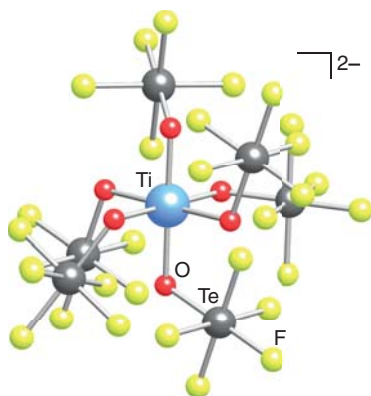
27 [\text{Ti}(\text{OTeF}_5)_6]^{2-}
