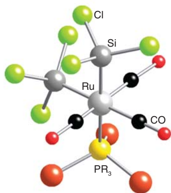
7 [\text{Ru}(\text{CO})_3(\text{SiCl}_3)_2(\text{PR}_3)]^+
