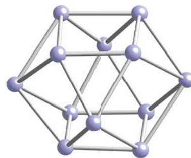
25 \text{B}_{12} cuboctahedron
