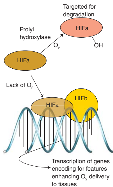
Figure 26.54 The principle of O_2 sensing by prolyl oxygenases.
