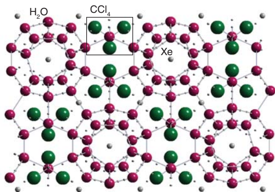
Figure 10.12 The cages of water molecules in clathrate hydrates, in this case \text{Xe}_4(\text{CCl}_4)_8(\text{H}_2\text{O})_{68} .
