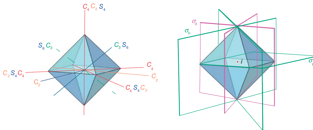
Figure 7.1* The highly symmetrical octahedral arrangement of six ligands around a central metal and the corresponding symmetry elements of an octahedron. Note that not all the \sigma_d are shown.
