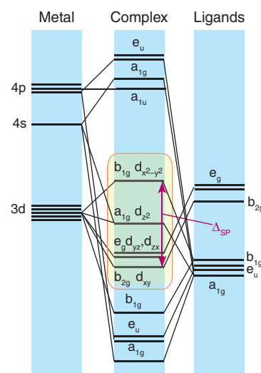
Figure 22.2 The energy levels of the molecular orbitals of a square-planar complex with strong-field ligands. The four lowest MOs correspond to bonding interactions, and the highest corresponds to an antibonding interaction; the MOs are labelled with the d orbitals from which they are derived.
