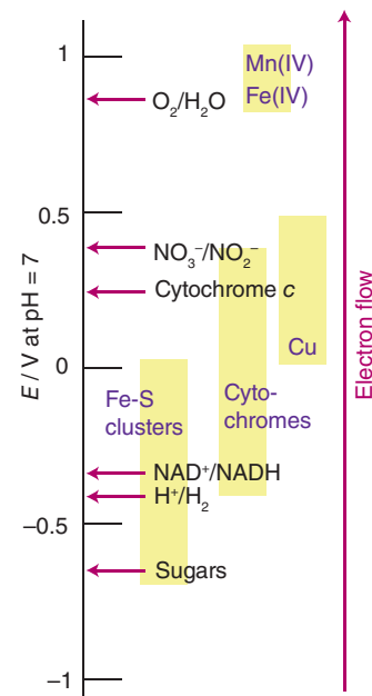
Figure 26.22 The 'redox spectrum' of life.
