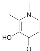
27 Deferiprone
