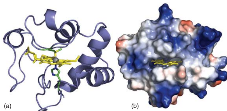
Figure 26.25* Different views (but from the same viewpoint) of mitochondrial cytochrome c : (a) the secondary structure and the position of the haem cofactor; (b) the surface charge distribution that guides the docking with its natural redox partners (red and blue areas represent patches of negative and positive charge, respectively).
