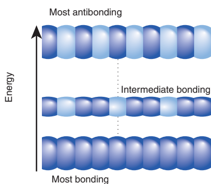
Figure 3.62 A band can be thought of as formed by bringing up atoms successively to form a line of atoms. N atomic orbitals give rise to N molecular orbitals.
