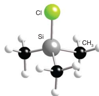
7 (CH_3)_3SiCl
