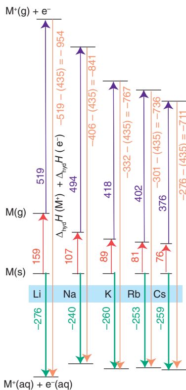
Figure 11.3 Thermochemical cycle (standard enthalpy changes in \text{kJ mol}^{-1} ) for the oxidation half-reaction M(s) \rightarrow M^+(aq) + e^-(aq) . A theoretical value of 435 \text{ kJ mol}^{-1} is included for the enthalpy of hydration of an electron, corresponding to the process \frac{1}{2} \text{H}_2(g) + \text{H}_2\text{O} \rightarrow \text{H}^+(aq) + e^-(aq) to allow the derived values for this half-reaction to be compared to the standard electrode potentials in Table 11.1.
