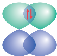
Figure 2.4 The formation of a \pi bond.
