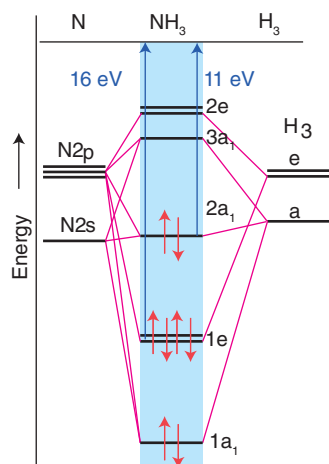
Figure 2.30 The molecular orbital energy-level diagram for \text{NH}_3 when the molecule has the observed bond angle ( 107^\circ ) and bond length.
