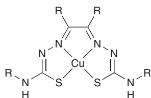
12 Cu-semithiocarbazonate complex
