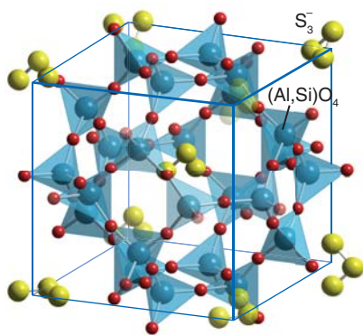
Figure 24.65* One of the sodalite cages present in ultramarine, \text{Na}_8[\text{SiAlO}_4]_6 \cdot (\text{S}_3)_2 . The framework consists of linked \text{SiO}_4 and \text{AlO}_4 tetrahedra surrounding a cavity containing the polysulfide radical ion \text{S}_3^- and \text{Na}^+ ions (the latter omitted for clarity).
