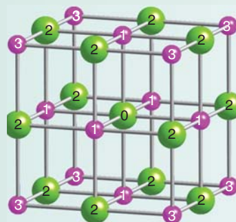
Figure B3.5 Basis for the calculation of the Madelung constant for the rock-salt structure type, showing the shells of ions at different distances from the central ion, labeled 0.
