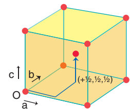
Figure 3.4 Lattice points describing the translational symmetry of a body-centred cubic unit cell. The translational symmetry is that of the unit cell and (+\frac{1}{2}, +\frac{1}{2}, +\frac{1}{2}) , so a lattice point at the origin, O, translates to the body centre of the unit cell.
