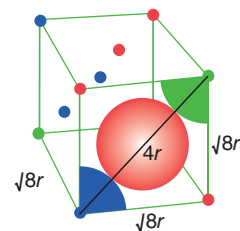
Figure 3.15 The dimensions involved in the calculation of the packing fraction in a close-packed arrangement of identical spheres of radius r .
