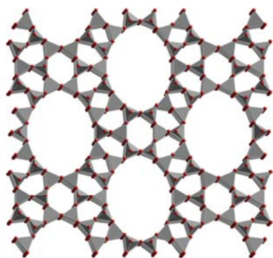
Figure 24.46* Representations as linked tetrahedra of synthesized zeolites showing the main channels in UTD-1.
