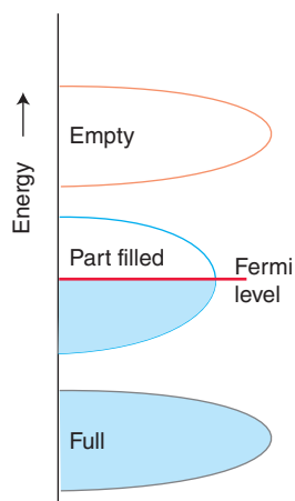
Figure 3.69 Typical density of states diagram for a three-dimensional metal.
