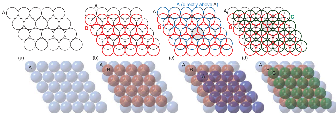
Figure 3.12* The formation of two close-packed polytypes. (a) A single close-packed layer, A. (b) The second close-packed layer, B, lies in dips above A. (c) The third layer reproduces the first to give an ABA structure (hcp). (d) The third layer lies above the gaps in the first layer, giving an ABC structure (ccp). The different colours identify the different layers of identical spheres.
