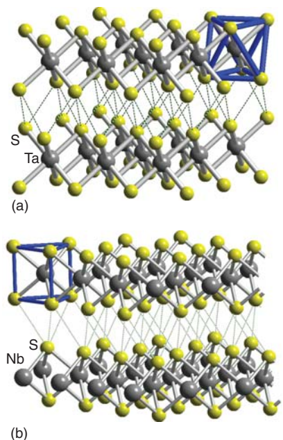
Figure 24.38* (a) The structure of \text{TaS}_2 ( \text{CdI}_2 -type); the Ta atoms reside in octahedral sites between the AB layers of S atoms. (b) The \text{NbS}_2 structure; the Nb atoms reside in trigonal prismatic sites, between the sulfide layers.
