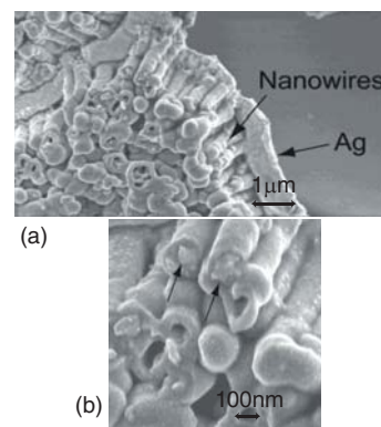
Figure 24.82 (a) Low-magnification and (b) high-magnification SEM images of Au/TiO 2 core-sheath nanowire arrays. (Y.-G. Guo, et al., J. Phys. Chem. B , 2003, 107 , 5441.).
