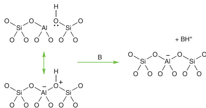
Figure 25.24 The Brønsted acid site in H-ZSM5 and its interaction with a base, typically an organic molecule. (Based on W.O. Haag, R.M. Lago, and P.B. Weisz, Nature , 1984, 309 , 589).
