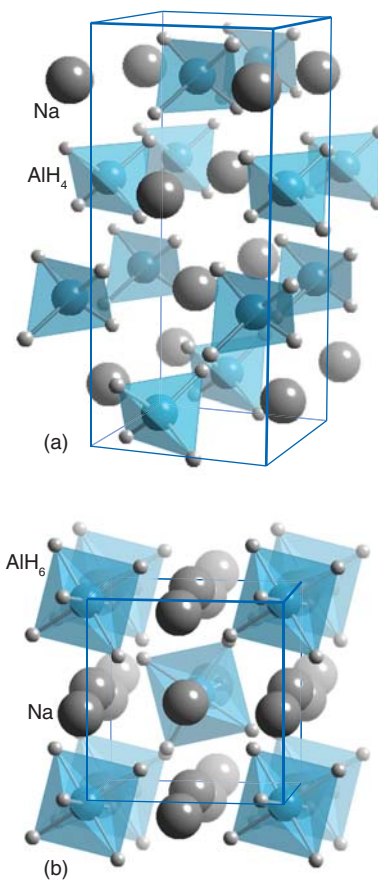
Figure 24.60 The structures of (a)* \text{NaAlH}_4 and (b)* \text{Na}_3\text{AlH}_6 , depicting the hydride coordination around aluminium.
