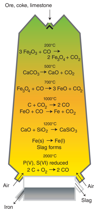
Figure 5.17 A schematic diagram of a blast furnace, showing the typical composition and temperature profile.
