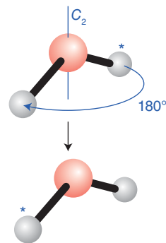
Figure 6.1* An \text{H}_2\text{O} molecule may be rotated through any angle about the bisector of the HOH bond angle, but only a rotation of 180^\circ (the C_2 operation) leaves it apparently unchanged.
