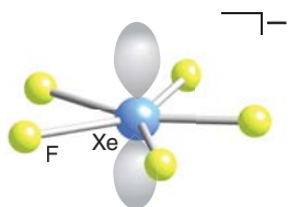
9 \text{XeF}_5^-
