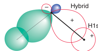
Figure 2.33 The formation of localized O–H orbitals in \text{H}_2\text{O} by the overlap of hybrid orbitals on the O atom and \text{H}1s orbitals. The hybrid orbitals are a close approximation to the \text{sp}^3 hybrids shown in Fig. 2.6.
