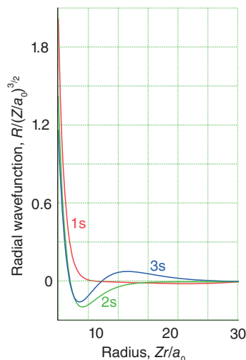
Figure 1.8 The radial wavefunctions of the 1s, 2s, and 3s hydrogenic orbitals. Note that the number of radial nodes is 0, 1, and 2, respectively. Each orbital has a nonzero amplitude at the nucleus (at r=0 ).
