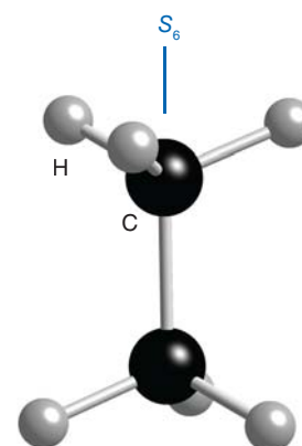
3 An S_6 axis
