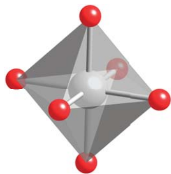
19 Octahedral complex, O_h
