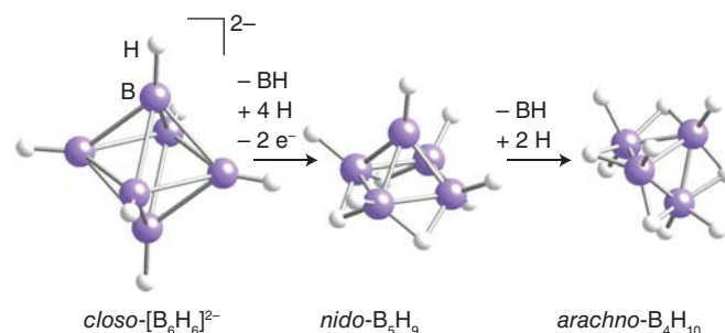
Figure 13.11 Structural correlations between a \text{B}_6 closo octahedral structure, a \text{B}_5 nido square pyramid, and a \text{B}_4 arachno butterfly.
