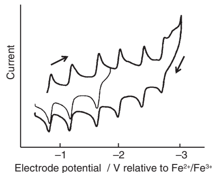
Figure 14.6 The cyclic voltammogram of C_{60} in DMF/toluene, recorded at low temperature. The reference electrode is ferrocene (Fc).
