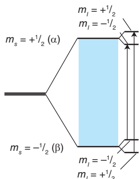
Figure 8.32 When a magnetic nucleus is present, its 2I+1 orientations give rise to a local magnetic field that splits each spin state of an electron into 2I+1 levels. The allowed transitions ( \Delta m_s = +1 , \Delta m_l = 0 ) give rise to the hyperfine structure of an EPR spectrum.
