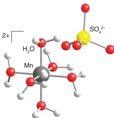
3 [\text{Mn}(\text{OH}_2)_6]\text{SO}_4
