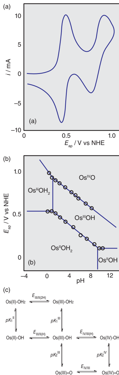
Figure 8.53 (a) Cyclic voltammetry of an Os(II) complex [Os II (bpy) 2 py(OH 2 )] 2+ (abbreviated as Os(OH 2 )) at pH 3.1 showing two one-electron processes generating first Os(III), then Os(IV) species. Sweep rate is 0.2 V/s. By carrying out the experiment over a wide pH range (0–10) the Pourbaix diagram (b) can be constructed (c) shows the possible elementary reactions that the Os(II) complex [Os II (bpy) 2 py(OH 2 )] 2+ can undergo during its oxidation at an electrode. Adapted from an original kindly supplied by Prof. J.-M. Saveant. Article published in Proc. Natl. Acad. Sci. USA. , 2009, 106 , 11829–11836.
