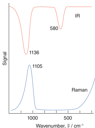
Figure 8.22 The IR and Raman spectra of XeF_4 .
