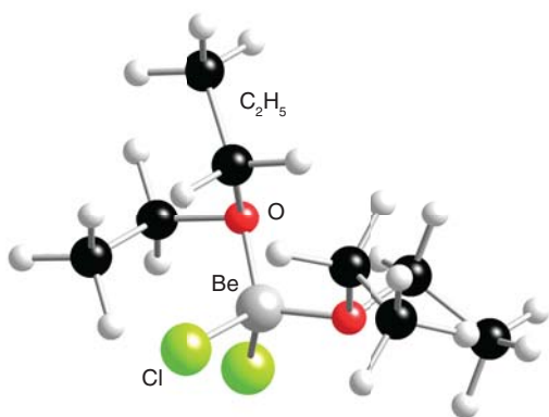
2 \text{BeCl}_2(\text{O}(\text{C}_2\text{H}_5)_2)_2
