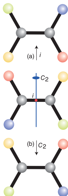
Figure 6.6* Care must be taken not to confuse (a) an inversion operation with (b) a two-fold rotation. Although the two operations may sometimes appear to have the same effect, that is not the case in general, as can be seen when the four terminal atoms of the same element are coloured differently.
