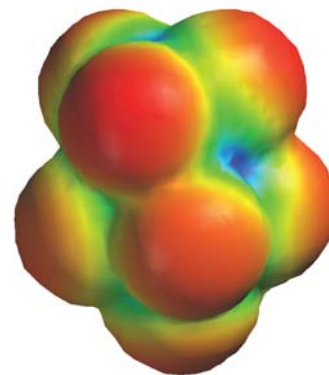
Figure 2.35 The output of computations of the electronic structure of a molecule is conveyed in a variety of ways. Here we show the electric potential surface of SF 5 CF 3 , a molecule that has been found to act as a very powerful greenhouse gas but is of uncertain origin in the atmosphere. Red areas indicate regions of negative potential and green regions of positive potential.
