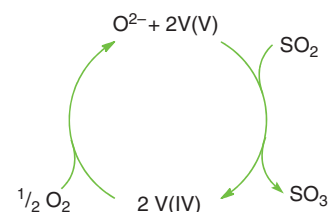
Figure 25.21 Cycle showing the key elements involved in the oxidation of SO 2 by V(V) compounds.
