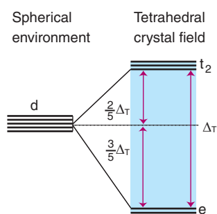
Figure 20.8 The orbital energy-level diagram used in the application of the building-up principle in a crystal-field analysis of a tetrahedral complex.
