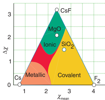
Figure 2.36 A Ketelaar triangle, showing how a plot of average electronegativity against electronegativity difference can be used to classify the bond type for binary compounds.
