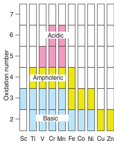
Figure 4.6 The oxidation numbers for which elements in the first row of the d block have amphoteric oxides. Predominantly acidic oxides are shown shaded pink, predominantly basic oxides are shaded blue.
