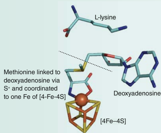
Figure B26.1 Structure of the active site of lysine 2,3-aminomutase, showing the arrangement of the precursor state in which S-adenosylmethionine is coordinated to the [4Fe-4S] cluster. Lysine, the substrate, is held close by.
