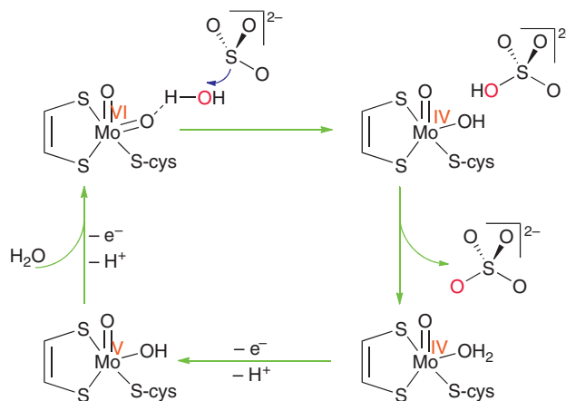
Figure 26.61 The mechanism referred to in Exercise 26.10.
