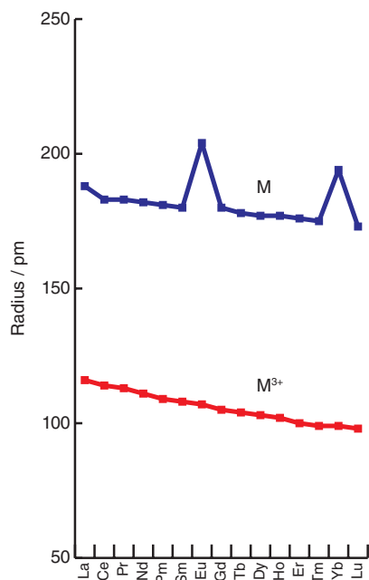
Figure 23.4 Variation of the metallic radii of Ln and ionic radii of \text{Ln}^{3+} .
