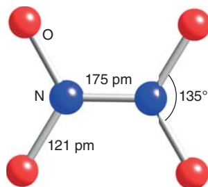
19 \text{N}_2\text{O}_4 , D_{2h}
