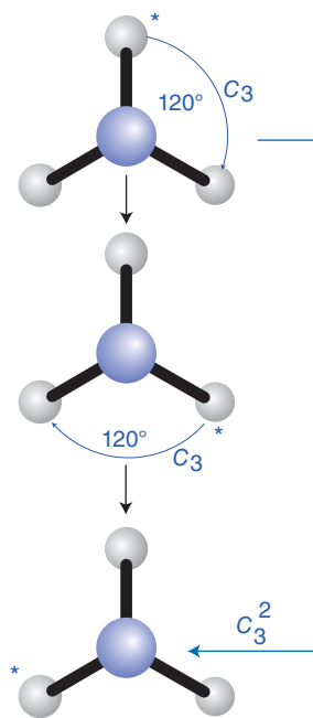
Figure 6.2* A three-fold rotation and the corresponding C_3 axis in \text{NH}_3 . There are two rotations associated with this axis, one through 120^\circ ( C_3 ) and one through 240^\circ ( C_3^2 ).
