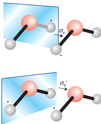
Figure 6.4* The two vertical mirror planes \sigma_v and \sigma_v' in H_2O and the corresponding operations. Both planes cut through the C_2 axis.
