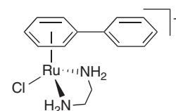
8 Half-sandwich Ru(II) arene complex
