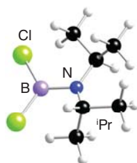
22 \text{Cl}_2\text{B-N}(\text{iPr})_2, \text{iPr} = (\text{CH}_3)_2\text{CH}
