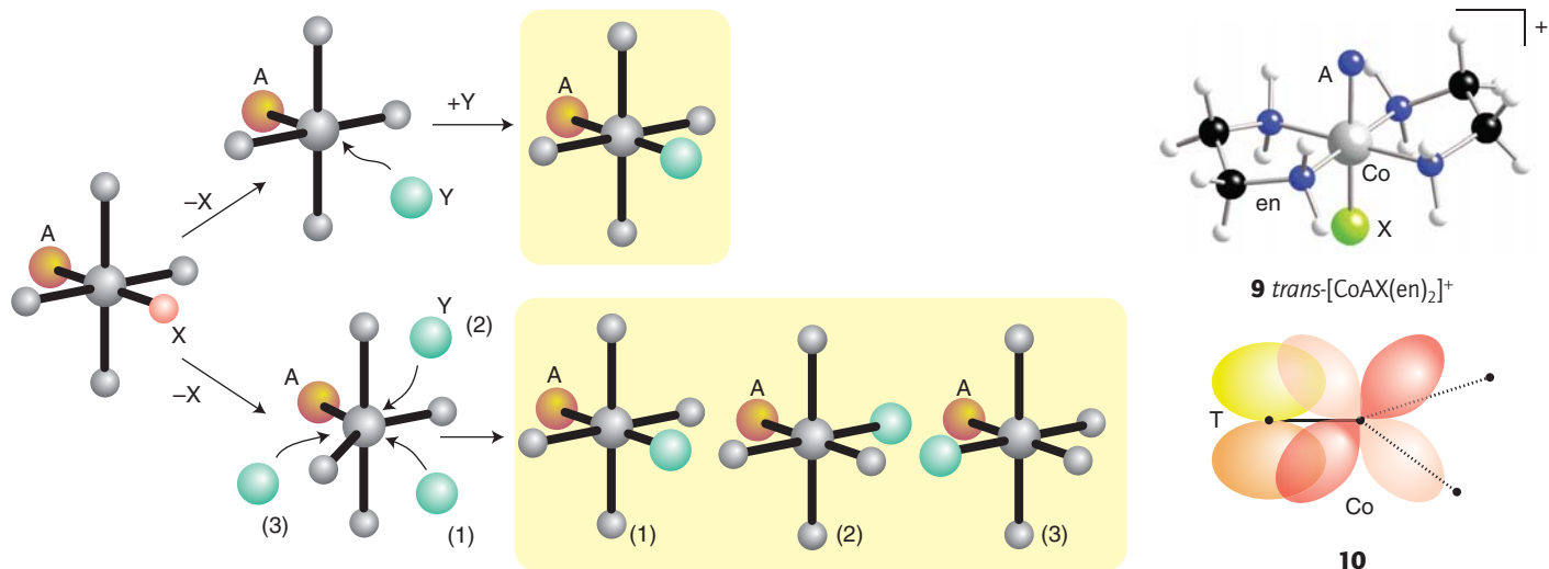
Figure 21.13* Reaction through a square-pyramidal complex (top path) results in retention of the original geometry, but reaction through a trigonal-bipyramidal complex (bottom path) can lead to isomerization.
