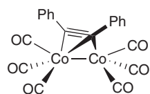
33 [\text{Co}_2(\text{PhC}\equiv\text{CPh})(\text{CO})_6]
