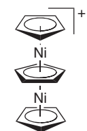
80 [\text{Ni}_2(\text{Cp})_3]^+
