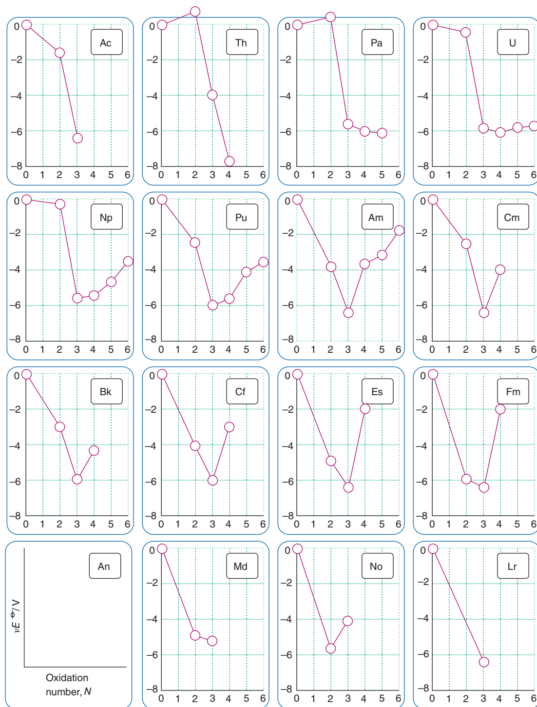
Figure 23.15 Frost diagrams of the actinoids in acidic solution. (Based on J.J. Katz, G.T. Seaborg, and L. Morss, Chemistry of the actinide elements . Chapman and Hall (1986).)
