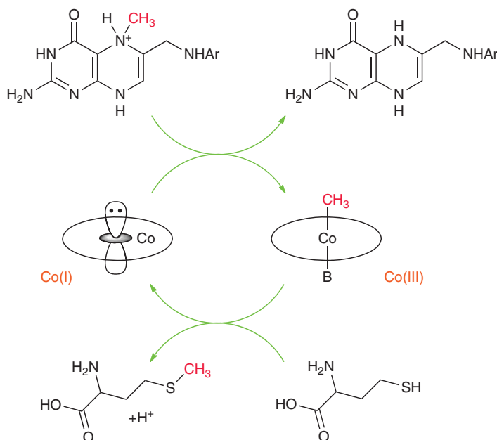
Figure 26.43 The mechanism of methionine synthase. Co(I) is a strong nucleophile and attacks the electrophilic quaternary-CH 3 group on the methyl carrier tetrahydrofolate. The resulting Co(III) methyl complex transfers CH 3 + to homocysteine.
