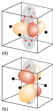
Figure 20.25* The shifts in electron density that accompany the two transitions discussed in the text. There is a considerable relocation of electron density towards the ligands on the z -axis in (a), but a much less substantial relocation in (b).
