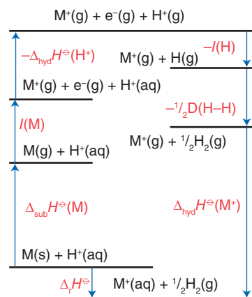
Figure 5.2 A thermodynamic cycle showing the properties that contribute to the standard potential of a metal couple. Endothermic processes are drawn with upward-pointing arrows and exothermic contributions with downward-pointing arrows.
