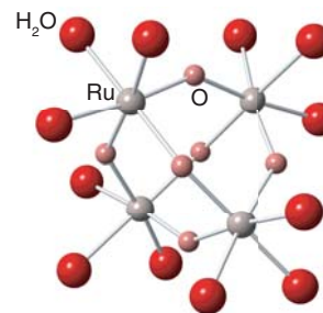
23 [\text{Ru}_4\text{O}_6(\text{H}_2\text{O})_{12}]^{4+}
