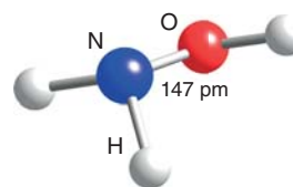
15 Hydroxylamine, \text{NH}_2\text{OH}
