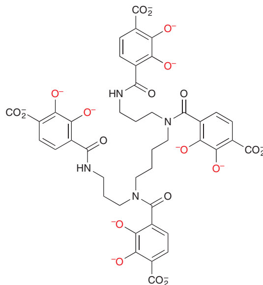
29 3,4,3-LIMACC
