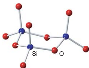
4 [\text{Si}_3\text{O}_9]^{6-}
