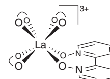
31 [\text{La}(\text{bpyO}_2)_4]^{3+}
