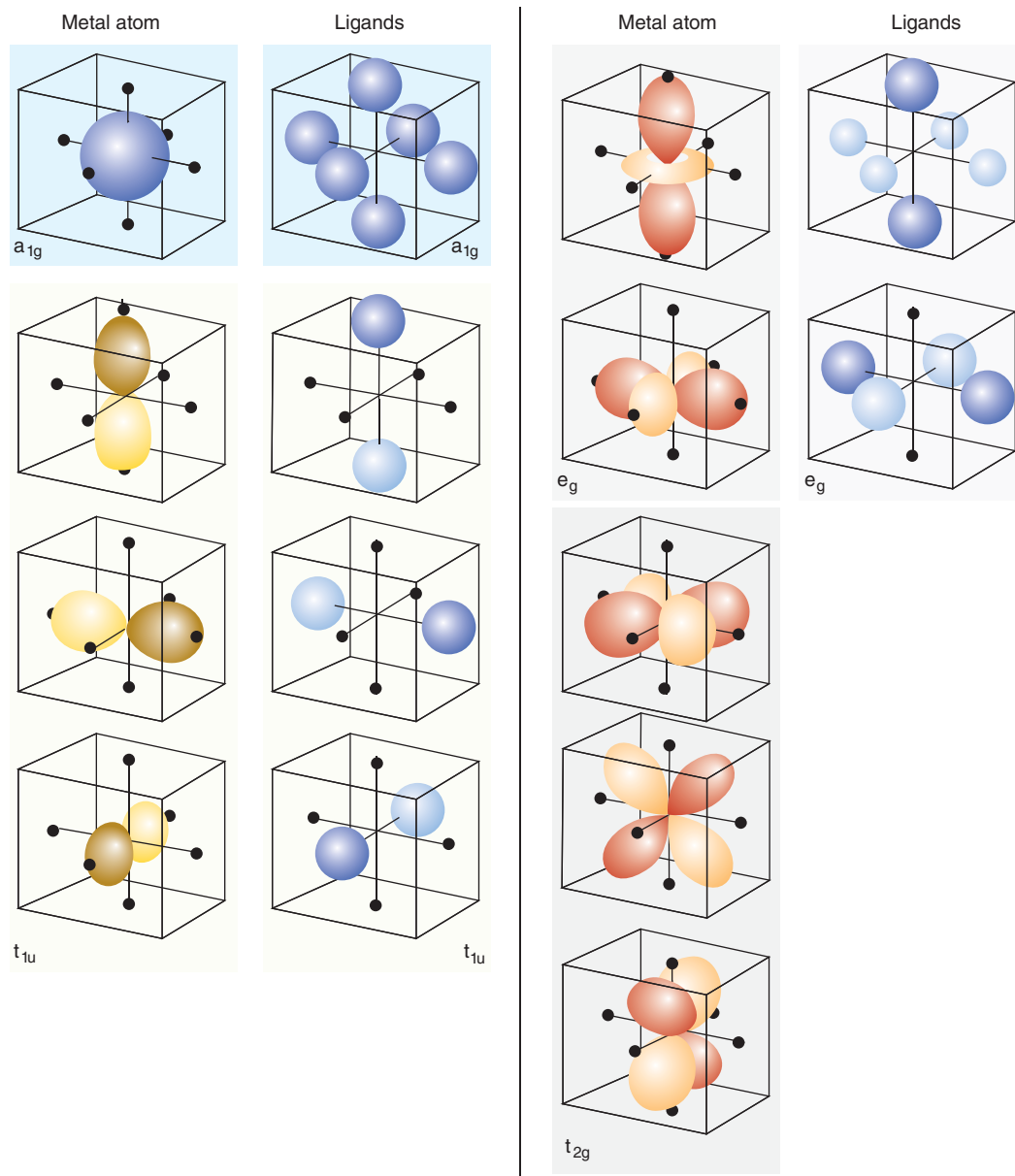
Figure 20.15* Symmetry-adapted combinations of ligand \sigma orbitals (represented here by spheres) in an octahedral complex. For symmetry-adapted orbitals in other point groups, see Resource section 5 .
