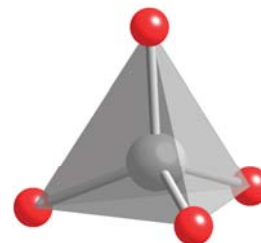
14 Tetrahedral complex, T_d
