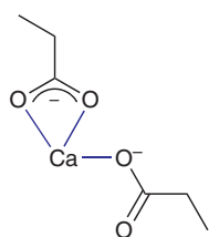
3 \text{Ca}^{2+} coordination
