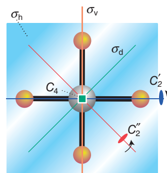
Figure 6.3* Some of the symmetry elements of a square-planar molecule such as \text{XeF}_4 .
