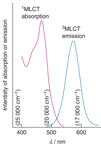
Figure 20.37 The absorption and phosphorescence spectra of [\text{Ru}(\text{bpy})_3]^{2+} .
