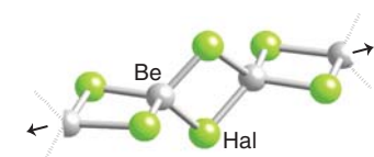
14 \text{Be}(\text{Hal})_2
