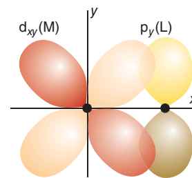
Figure 20.19* The \pi overlap that may occur between a ligand p orbital perpendicular to the M–L axis and a metal d_{xy} orbital.
