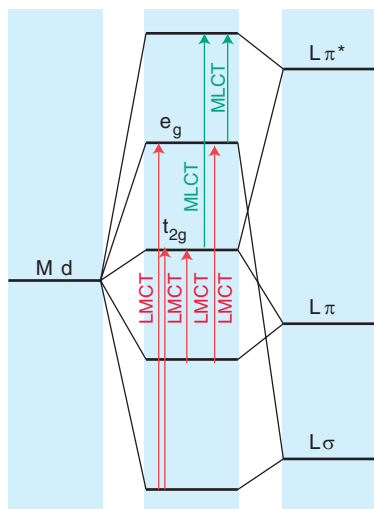
Figure 20.32 A summary of the charge-transfer transitions in an octahedral complex.
