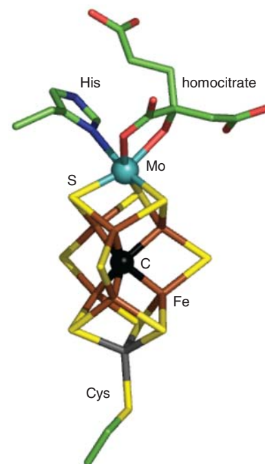
51* Nitrogenase ‘FeMoco’ [ \text{Mo}_7\text{Fe}_9\text{S} , C]
