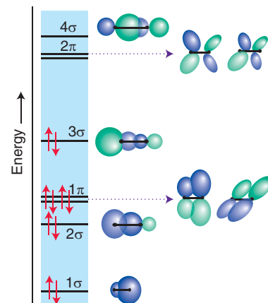
Figure 2.23 A schematic illustration of the molecular orbitals of CO, with the size of the atomic orbital indicating the magnitude of its contribution to the molecular orbital.
