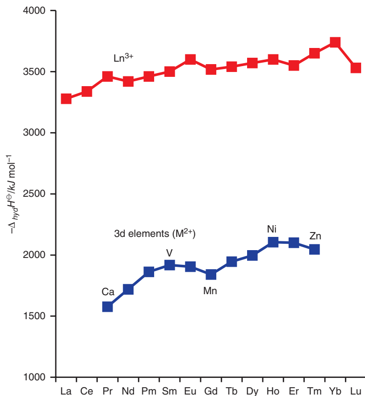
Figure 23.5 Enthalpies of hydration of \text{Ln}^{3+} ions and comparison with \text{M}^{2+} cations of the 3d metals.
