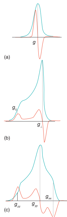
Figure 8.31 The forms of EPR powder (frozen solution) spectra expected for different types of g -value anisotropy (a), (b) and (c). The blue line is the absorption and the red line the first derivative of the absorption (its slope). For technical reasons related to the detection technique, the first derivative is normally observed in EPR spectrometers.
