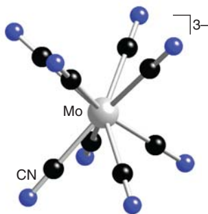
28 [\text{Mo}(\text{CN})_8]^{3-}
