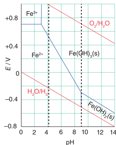
Figure 5.11 A simplified Pourbaix diagram for some important naturally occurring aqua species of iron. The broken black vertical lines represent the normal pH range in natural waters.
