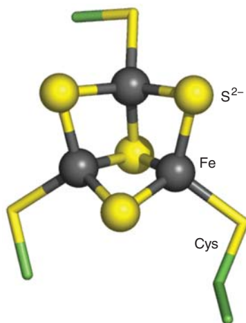
27* [3Fe-4S]
