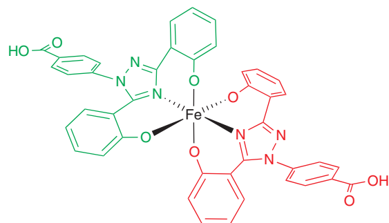
28 [\text{Fe(III)}(\text{deferasirox})_2]^-
