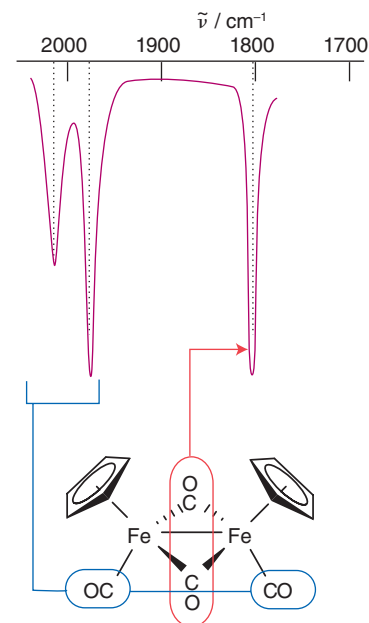
Figure 22.12 The infrared spectrum of [\text{Fe}_2(\text{Cp})_2(\text{CO})_4] . Note the two high-frequency terminal CO stretches and the lower-frequency absorption of the bridging CO ligands. Although two bridging CO bands would be expected on account of the low symmetry of the complex, a single band is observed because the two bridging CO groups are nearly collinear.
