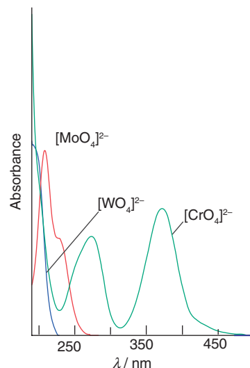
Figure 20.34 Optical absorption spectra of the ions [\text{CrO}_4]^{2-} , [\text{WO}_4]^{2-} , and [\text{MoO}_4]^{2-} . On descending the group, the absorption maximum moves to shorter wavelengths, indicating an increase in the energy of the LMCT band.
