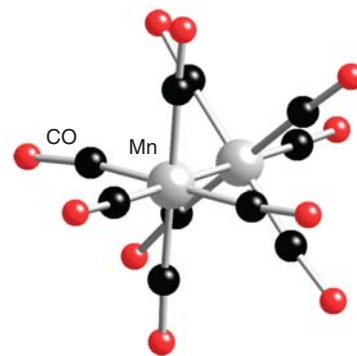
37 [(\text{OC})_5\text{Mn}-\text{Mn}(\text{CO})_5]
