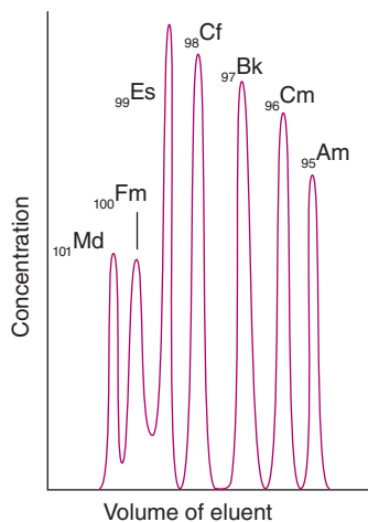
Figure 23.14 Elution of heavy actinoid ions from a cation exchange column using ammonium 2-hydroxyisobutyrate as the eluent. Note the similarity in elution sequence to Fig. 23.13: the heavy (smaller) \text{An}^{3+} ions elute first.
