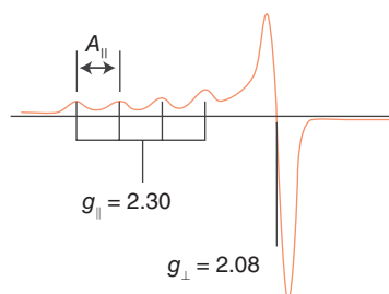
Figure 8.33 The EPR spectrum of \text{Cu}^{2+} ( d^9 , one unpaired electron) in frozen aqueous solution. The tetragonally distorted \text{Cu}^{2+} ion shows an axially symmetrical spectrum in which hyperfine coupling to Cu ( I = \frac{3}{2} , four hyperfine lines) is clearly evident for the g_{\parallel} component.
