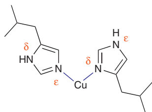
4 Cu-imidazole coordination
