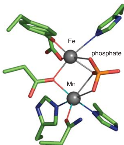
34* Active site of an acid phosphatase
