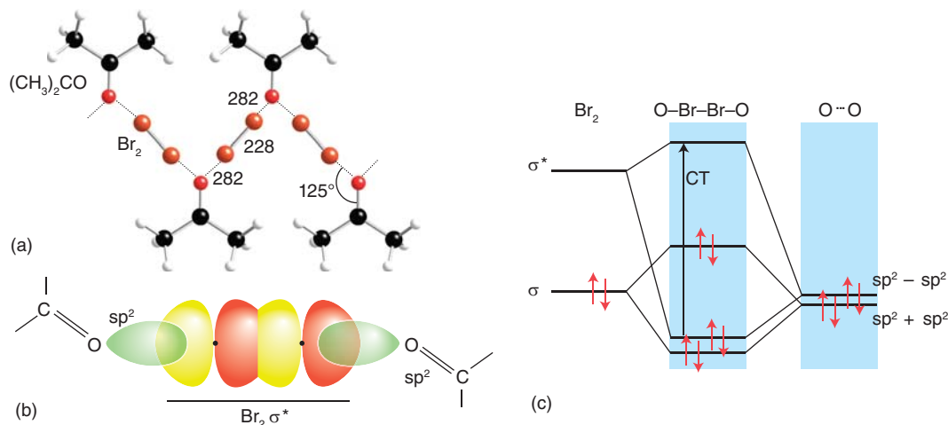
Figure 4.10* The interaction of \text{Br}_2 with the carbonyl group of propanone. (a) The structure of (\text{CH}_3)_2\text{COBr}_2 shown by X-ray diffraction. (b) The orbital overlap responsible for the complex formation. (c) A partial molecular orbital energy-level diagram for the \sigma and \sigma^* orbitals of \text{Br}_2 with the appropriate combinations of the \text{sp}^2 orbitals on the two O atoms. The charge-transfer transition is labelled CT.
