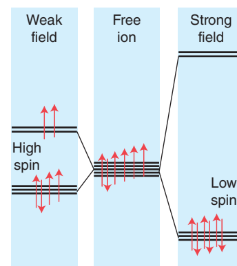
Figure 20.5 The effect of weak and strong ligand fields on the occupation of orbitals for a d 6 complex. The former results in a high-spin configuration and the latter in a low-spin configuration.
