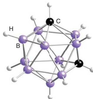
36 closo -1,7- B_{10}C_2H_{12}
