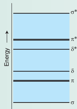
Figure B19.5 Approximate molecular orbital energy-level scheme for the M—M interactions in a quadruply bonded system, where only the d_{x^2-y^2} is used in bonding to the ligands.
