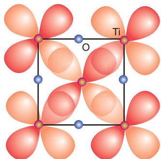
Figure 24.11 Overlap of the d_{zx} orbitals in TiO to give a t_{2g} band. In the perpendicular directions the d_{yx} and d_{xy} orbitals overlap in an identical manner.
