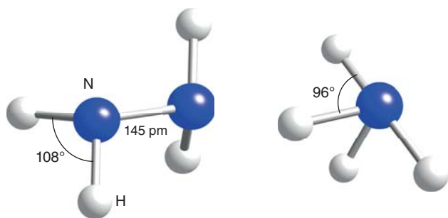
14 Hydrazine, \text{N}_2\text{H}_4
