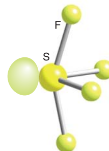
14 \text{SF}_4
