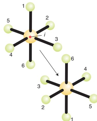
Figure 6.5* The inversion operation and the centre of inversion i in SF_6 .
