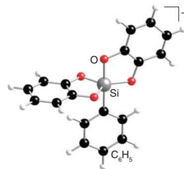
17 [\text{Si}(\text{C}_6\text{H}_5)(\text{OC}_6\text{H}_4\text{O})_2]^-
