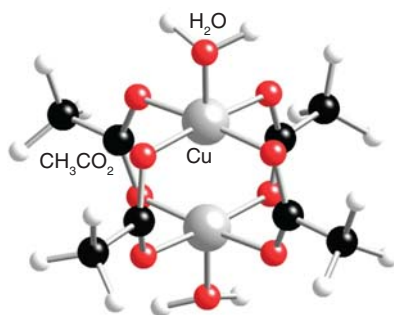
34 [(\text{H}_2\text{O})\text{Cu}(\mu\text{-CH}_3\text{CO}_2)_4\text{Cu}(\text{OH}_2)]
