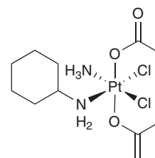
5 Satraplatin
