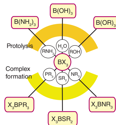
Figure 13.3 The reactions of boron–halogen compounds (X=halogen).
