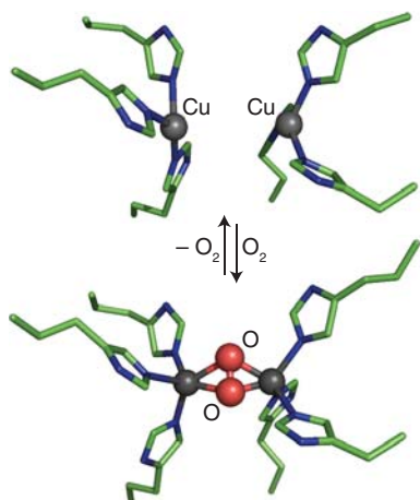
Figure 26.20* Binding of O_2 at the active site of haemocyanin causes the two Cu atoms to be brought closer together. The O_2 complex is regarded as a binuclear Cu(II) centre in which the two Cu atoms are bridged by an \eta^2, \eta^2 -peroxide.
