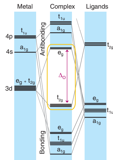
Figure 22.1 The energy levels of the molecular orbitals of an octahedral complex with strong-field ligands.
