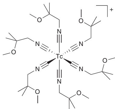
31 Cardiolyte (heart)
