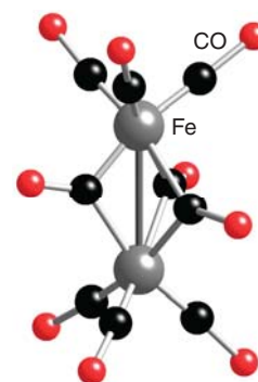
83 [\text{Fe}_2(\text{CO})_9]
