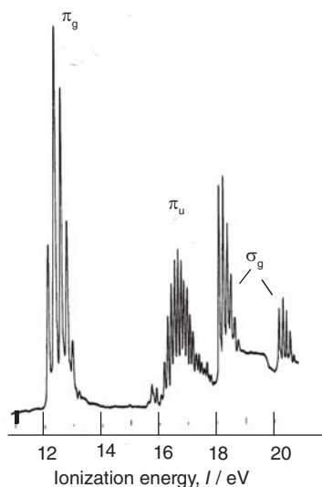
Figure 8.37 The UV photoelectron spectra of O_2 . Loss of an electron from 2\sigma_g (see the MO energy-level diagram, Fig. 2.12) gives rise to two bands because the unpaired electron that remains can be parallel or antiparallel to the two unpaired electrons in the 1\pi_g orbitals.
