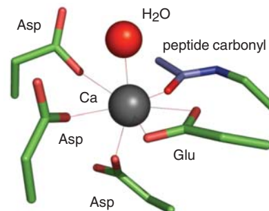
12* A \text{Ca}^{2+} -binding site in calmodulin
