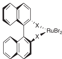
8 [Ru(BINAP)Br 2 ]. X = PPh 2
