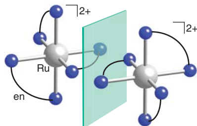
76 [\text{Ru}(\text{en})_3]^{2+} enantiomers
