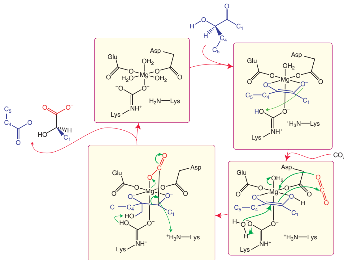
Figure 26.32 Mechanism of action of ribulose 1,5-bisphosphate carboxylase, the enzyme responsible for removing \text{CO}_2 from the atmosphere and 'fixing' it in organic molecules in plants.
