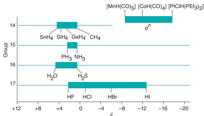
Figure 10.4 Typical ^1\text{H} -NMR chemical shifts. The tinted boxes show families of elements together.
