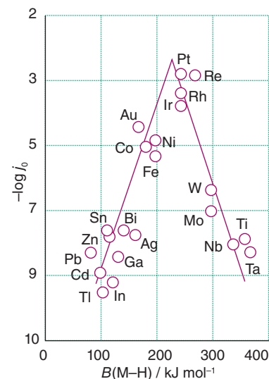
Figure 25.25 The rate of \text{H}_2 evolution expressed as the logarithm of the exchange current density plotted against \text{M}-\text{H} bond energy.
