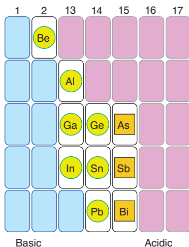
Figure 4.5 The location of elements having amphoteric oxides. The circled elements have amphoteric oxides in all oxidation states. The elements in boxes have acidic oxides in the highest oxidation state and amphoteric oxides in lower oxidation states.
