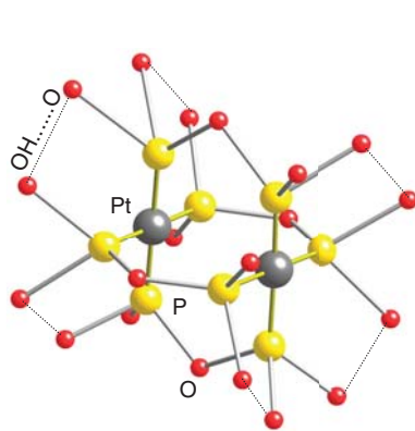
21 [\text{Pt}_2(\mu\text{-P}_2\text{O}_5\text{H}_2)_4]^{4-} , PtPOP
