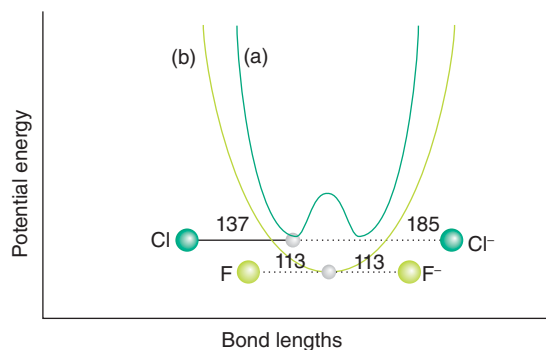
Figure 10.9 The variation of the potential energy with the position of the proton between two atoms in a hydrogen bond: (a) the double-minimum potential characteristic of a weak hydrogen bond; (b) the single-minimum potential characteristic of a strong hydrogen bond.
