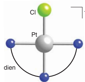
77 [\text{PtCl}(\text{dien})]^+
