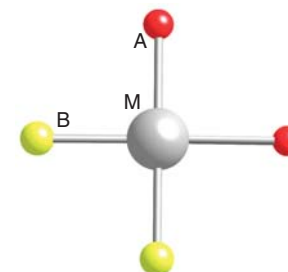
40 cis - [\text{MA}_2\text{B}_2]
