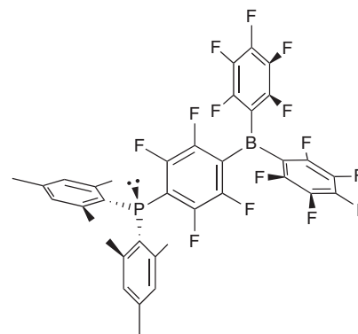
22 (\text{C}_6\text{H}_2\text{Me}_3)_2\text{P}(\text{C}_6\text{F}_4)\text{B}(\text{C}_6\text{F}_5)_2
