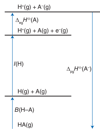
Figure 4.2 Thermodynamic cycle for a proton-gain reaction.
