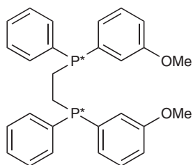
6 DiPAMP
