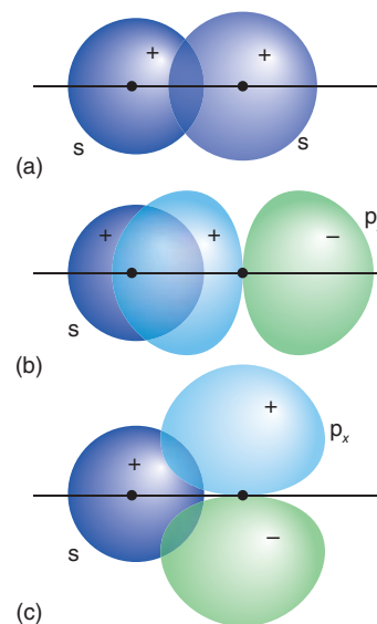
Figure 6.20* An s orbital can overlap (a) an s or (b) a p_z orbital on a second atom with constructive interference. (c) An s orbital has zero net overlap with a p_x or p_y orbital because the constructive interference between the parts of the atomic orbitals with the same sign exactly matches the destructive interference between the parts with opposite signs.
