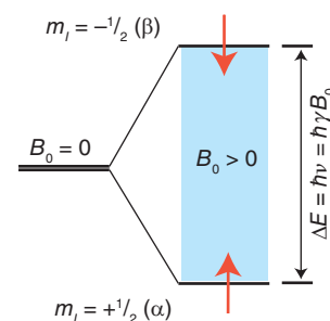
Figure 8.23 When a nucleus with spin I > 0 is in a magnetic field, its 2I+1 orientations (designated m_I ) have different energies. This diagram shows the energy levels of a nucleus with I = \frac{1}{2} (as for ^1\text{H} , ^{13}\text{C} , ^{31}\text{P} ).
