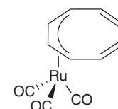
38 [\text{Ru}(\eta^4\text{-C}_8\text{H}_8)(\text{CO})_3]
