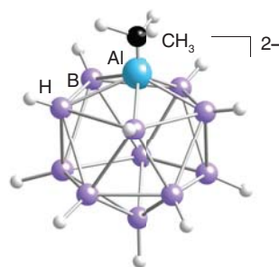
30 closo - [\text{B}_{11}\text{H}_{11}\text{AlCH}_3]^{2-}
