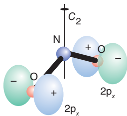
Figure 6.22* The combination of O2p x orbitals referred to in Example 6.11.
