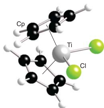
78 [\text{Ti}(\text{Cp})_2\text{Cl}_2]
