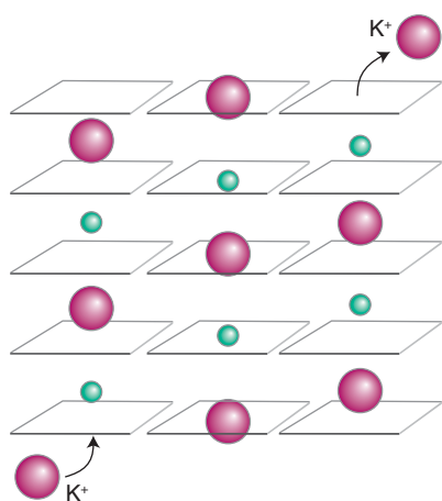
Figure 26.6 Mechanism of transport of K^+ ions through the selectivity filter of the K^+ channel. Green spheres represent water molecules.
