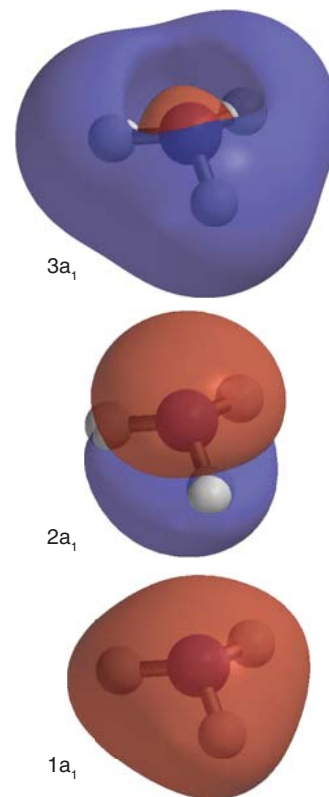
Figure 6.23* The three a_1 molecular orbitals of \text{NH}_3 as computed by molecular modelling software.
