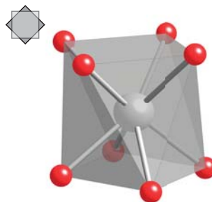
26 Square antiprism, D_4
