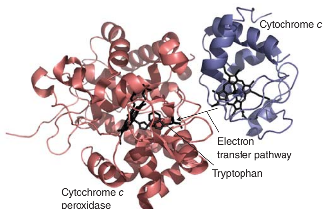
Figure 26.26* The bimolecular ET complex between cytochrome c and cytochrome c peroxidase produced by co-crystallization of cytochrome c with the Zn derivative of cytochrome c peroxidase. The orientation suggests an electron-transfer pathway between the haem groups of cytochrome c and cytochrome c peroxidase that includes tryptophan.
