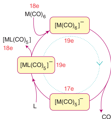
Figure 22.17 Schematic diagram of an electron-transfer catalysed CO substitution. After addition of a small amount of a reducing initiator, the cycle continues until the limiting reagent, [\text{M}(\text{CO})_6] or L, has been consumed.
