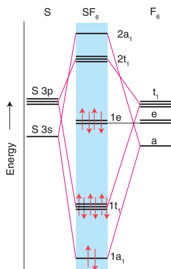
Figure 2.31 A schematic molecular orbital energy-level diagram for \text{SF}_6 .
