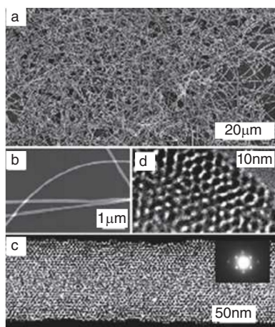
Figure 24.92 (a) SEM image of mesoporous silica nanofibres. (b) Low-magnification TEM image of the nanofibres. (c) High-magnification TEM image of one nanofibre; the inset is a selected-area electron diffraction pattern of the nanofibre. (d) High-resolution TEM image recorded at the edge of one nanofibre. (J. Wang, et al., Chem. Mater. , 2004, 16, 5169.)
