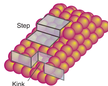
Figure 25.19 Schematic representation of surface irregularities, steps, and kinks.
