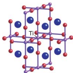
Figure 3.43 The local coordination environment of a Ti atom in perovskite.
