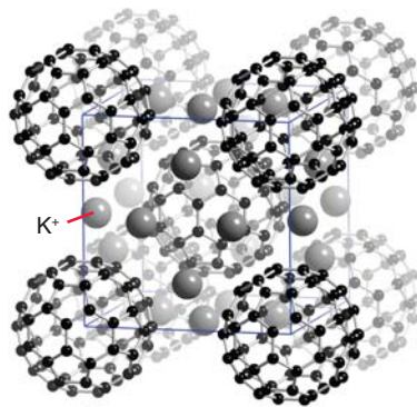
Figure 24.69* The structure of K_6C_{60} , with a body-centred cubic unit cell with C_{60}^{6-} molecular ions at the cell corners and body centre, and K^+ ions occupying half of the sites in the faces of the cell which have approximate tetrahedral coordination to four C_{60} molecular ions.
