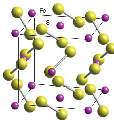
Figure 16.4 The structure of pyrite, FeS_2 .
