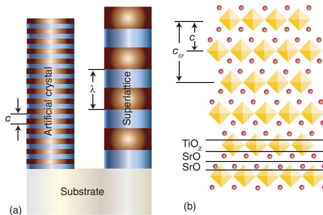
Figure 24.85 (a) The structure of an AB artificial crystal and an AB superlattice; c and \lambda represent the repeat periods during growth of the artificial structure and the superlattice period, respectively. (b) The structure of \text{Sr}_2\text{TiO}_4 as an artificially layered oxide. The polyhedra represent Ti-centred, corner-sharing \text{TiO}_6 octahedra and the spheres represent \text{Sr}^{2+} cations. The lateral coherency between the SrO and \text{TiO}_2 sublayers is excellent in this layered structure and the crystallographic repeat parameter, c_{cr} , is twice the growth repeat period, c .
