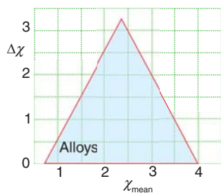
Figure 3.25 The approximate locations of alloys in a Ketelaar triangle.
