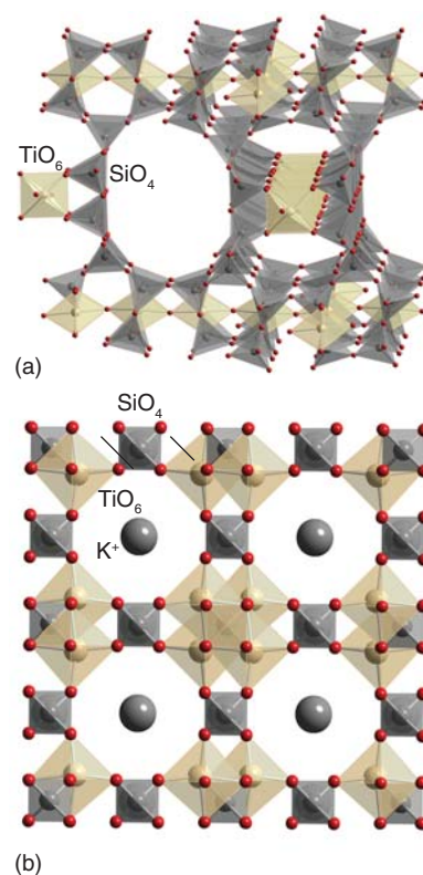
Figure 24.54 The structures of (a)* the titanosilicate ETS-10, which is built from chains of \text{TiO}_6 octahedra linked by \text{SiO}_4 tetrahedra, and (b)* \text{K}_3\text{H}(\text{TiO})_4(\text{SiO}_4)_3 \cdot 4\text{H}_2\text{O} , a synthetic analogue of a natural mineral, pharmacosiderite.
