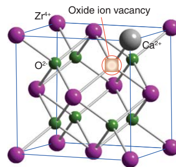
Figure 3.56* Introduction of a \text{Ca}^{2+} ion into the \text{ZrO}_2 lattice produces a vacancy on the \text{O}^{2-} sublattice. This substitution helps to stabilize the cubic fluorite structure for \text{ZrO}_2 .
