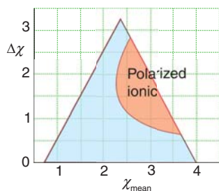
Figure 3.37 The location of polarized ionic salts in a Ketelaar triangle.
