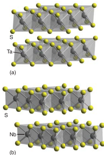
Figure 24.39* The metal-disulfide structures of Figure 24.38 drawn as layers of \text{MS}_6 polyhedra sharing edges: (a) octahedra in \text{TaS}_2 , (b) trigonal prisms in \text{NbS}_2 .
