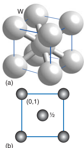
Figure 3.8 (a)* The structure of metallic tungsten and (b) its projection representation.
