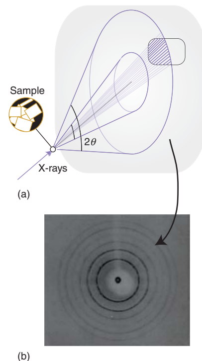
Figure 8.2 (a) The cones of diffraction that result from X-ray scattering by a powdered sample. The cone consists of thousands of individual diffraction spots, from individual crystallites, that merge together. (b) A photographic image of the diffraction pattern from a powdered sample. The undiffracted straight-through beam is at the centre of the image and the various diffraction cones, corresponding to different d -spacings, are observed as concentric circles.
