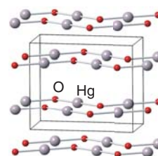
Figure 19.9* The structure of \text{HgO} .
