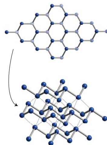
Figure 15.2 The structure of bismuth. In each puckered layer (upper diagram), every Bi atom has three nearest neighbours; three weaker interactions exist with Bi atoms in an adjacent sheet.
