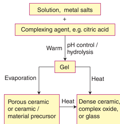
Figure 24.1 Schematic diagram of the Pechini sol-gel process. When the gel is dried at high temperatures, dense ceramics or glasses are formed. Drying at low temperatures above the critical pressure of water produces porous solids known as xerogels or aerogels.
