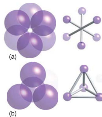
Figure 3.17 (a) An octahedral hole and (b) a tetrahedral hole formed in an arrangement of close-packed spheres.
