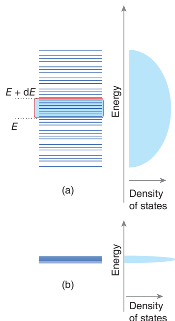
Figure 3.68 (a) The density of states in a metal is the number of energy levels in an infinitesimal range of energies between E and E + dE . (b) The density of states associated with a low concentration of dopant.
