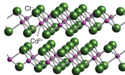
Figure 3.41* The \text{CdCl}_2 structure.
