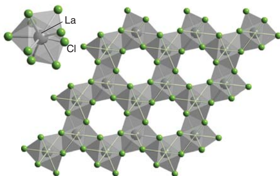
Figure 23.9* The structure of \text{LaCl}_3 shown as vertex-linked \text{LaCl}_3 -capped antiprisms: a single unit is shown as inset.
