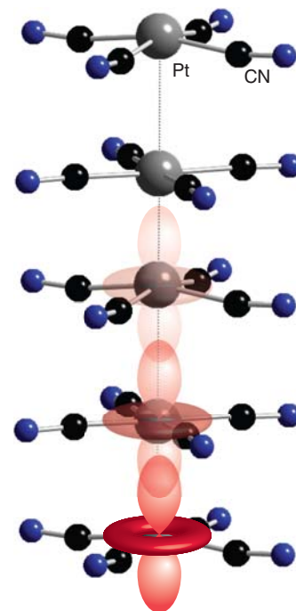
Figure 24.71* A representation of the infinite-chain structure of KCP ( \text{K}_2\text{Pt}(\text{CN})_4\text{Br}_{0.3} \cdot 3\text{H}_2\text{O} ) and a schematic illustration of its d band.
