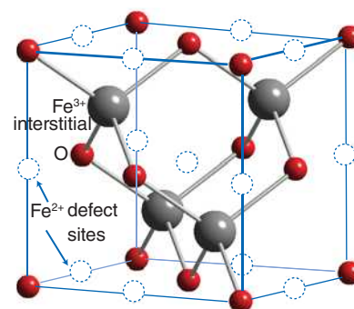
Figure 24.10 Defect sites proposed for Fe_{1-x}O . Note that the tetrahedral Fe^{3+} interstitials (grey spheres) and octahedral Fe^{2+} vacancies (circles) are clustered together.
