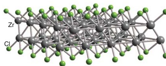
Figure 19.3* The structure of \text{ZrCl} consists of layers of metal atoms in graphite-like hexagonal nets.
