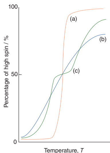
Figure 20.43 The change to high-spin might be (a) abrupt, (b) gradual, or (c) stepped.
