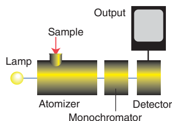
Figure 8.44 The layout of a typical atomic absorption spectrophotometer.
