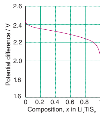
Figure 24.41 A diagram of potential versus composition for the electrointercalation of lithium into titanium disulfide. The composition, x , in \text{Li}_x\text{TiS}_2 is calculated from the charge passed in the course of electrointercalation.
