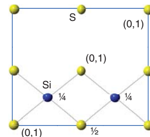
Figure 3.10* The structure of silicon sulfide ( \text{SiS}_2 ).
