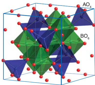
Figure 24.18* A segment of the spinel ( \text{AB}_2\text{O}_4 ) unit cell, showing the tetrahedral environment of A ions and the octahedral environments of B ions (compare this with Fig. 3.44).
