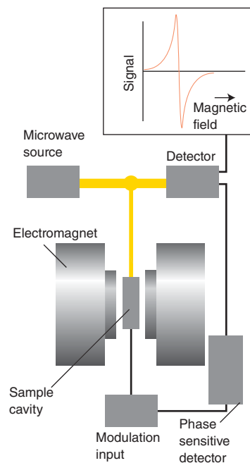
Figure 8.30 The layout of a typical continuous wave EPR spectrometer.
