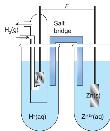
Figure 5.1 A schematic diagram of a galvanic cell. The standard potential, E_{\text{cell}}^\ominus , is the potential difference when the cell is not generating current and all the substances are in their standard states.
