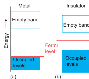
Figure 3.67 (a) Typical band structure for a metal showing the Fermi level; if each of the N atoms supplies one s electron, then at T=0 the lower \frac{1}{2}N orbitals are occupied and the Fermi level lies near the centre of the band. (b) Typical band structure for an insulator with the Fermi level midway in the band gap.
