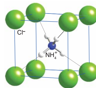
Figure 3.33* The structure of ammonium chloride, \text{NH}_4\text{Cl} , reflects the ability of the tetrahedral \text{NH}_4^+ ion to form hydrogen bonds to the tetrahedral array of \text{Cl}^- ions around it.
