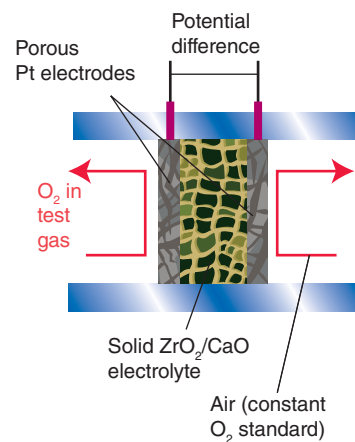
Figure 24.9 An oxygen sensor based on the solid electrolyte \text{Zr}_{1-x}\text{Ca}_x\text{O}_{2-x} .
