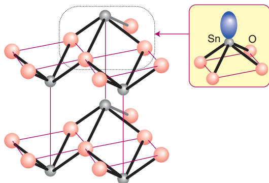
Figure 14.12 The structure of blue-black SnO, showing parallel layers of square-based pyramidal \text{SnO}_4 units.
