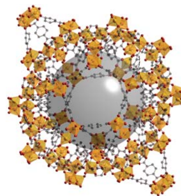
Figure 24.58* A metal–organic framework (MOF) formed from chromium terephthalate units showing \text{CrO}_6 octahedra (gold) linked by the organic anions. The large central sphere shows the extent of the pore in this material, which can be filled with solvent or gas molecules.
