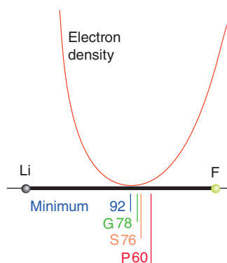
Figure 3.46 The variation in electron density along the Li-F axis in LiF. The point P indicates the Pauling radii of the two ions, G the original (1927) Goldschmidt radii, and S the Shannon radii ( Resource section 1 ).
