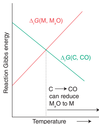
Figure 5.14 The variation of the standard reaction Gibbs energies for the formation of a metal oxide and carbon monoxide with temperature. The formation of carbon monoxide from carbon can reduce the metal oxide to the metal at temperatures higher than the point of intersection of the two lines. More specifically, at the intersection the equilibrium constant changes from K < 1 to K > 1 . This type of display is an example of an Ellingham diagram .
