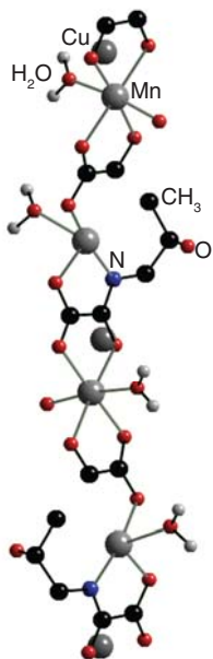
6 \text{MnCu}(\text{2-hydroxy-1,3-propenebisoxamato}) \cdot 3\text{H}_2\text{O}
