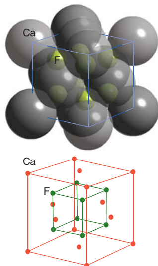
Figure 12.2* The fluorite structure adopted by \text{CaF}_2 , \text{SrF}_2 , \text{BaF}_2 , and \text{SrCl}_2 .
