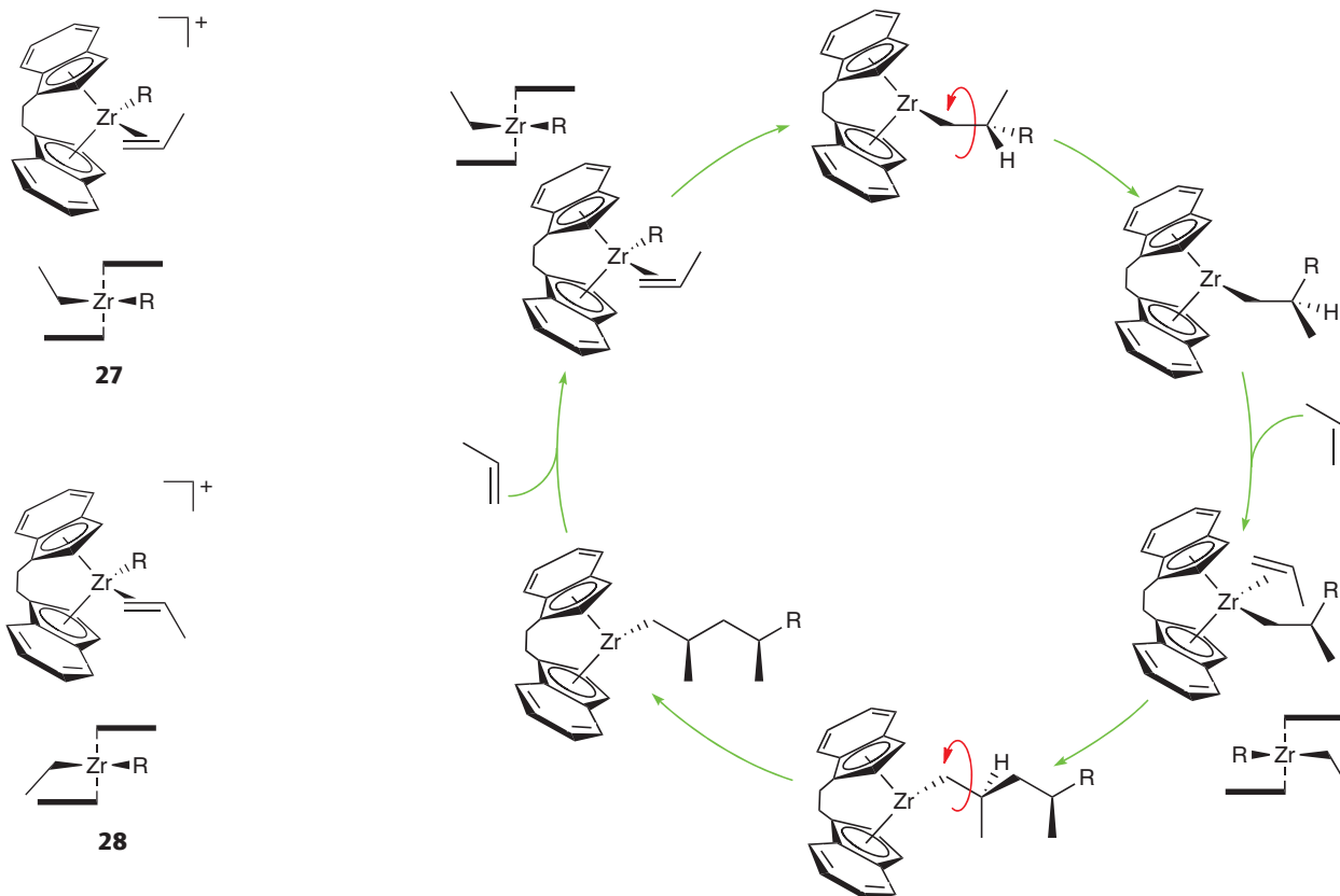
Figure 25.27 When propene is polymerized with an indenyl metallocene catalyst, isotactic polypropene results. The zirconium species all have a single positive charge; this has been omitted for clarity.
