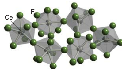
Figure 23.10* The structure of \text{CeF}_4 contains vertex-sharing \text{CeF}_8 antiprisms.
