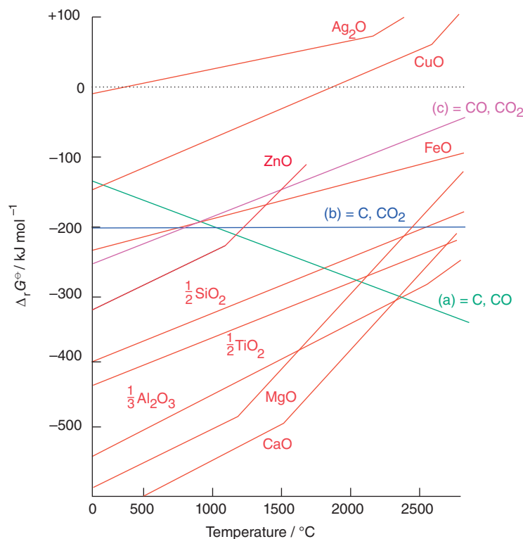
Figure 5.16 An Ellingham diagram for the reduction of metal oxides.
