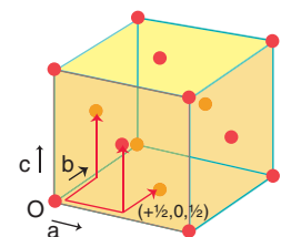
Figure 3.5 Lattice points describing the translational symmetry of a face-centred cubic unit cell. The translational symmetry is that of the unit cell and (+\frac{1}{2}, +\frac{1}{2}, 0) , (+\frac{1}{2}, 0, +\frac{1}{2}) , and (0, +\frac{1}{2}, +\frac{1}{2}) so a lattice point at the origin, O, translates to points in the centres of each of the faces.
