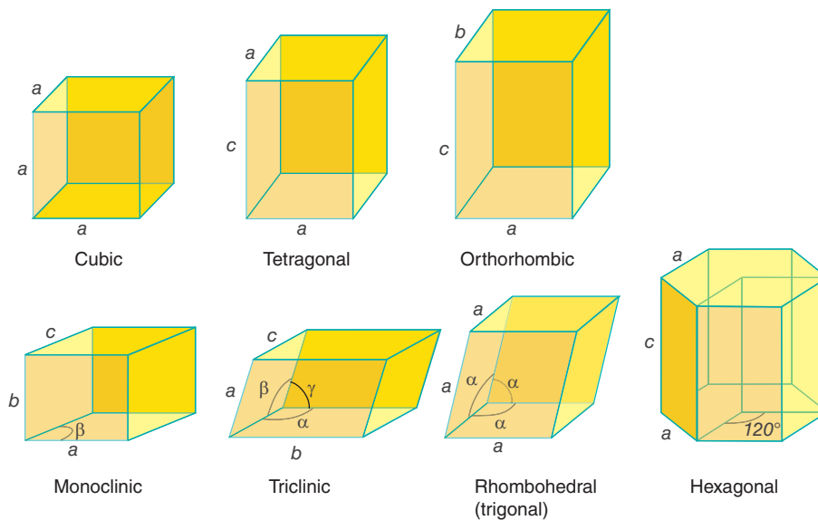
Figure 3.2 The seven crystal systems.
