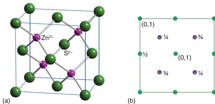
Figure 3.34 (a)* The sphalerite (zinc-blende) structure and (b) its projection representation. Note its relation to the ccp lattice in Fig. 3.18a, with half the tetrahedral holes occupied by \text{Zn}^{2+} ions.
