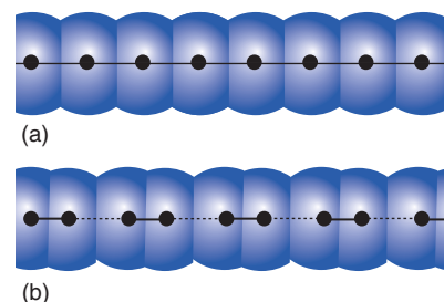
Figure 24.72 The formation of a Peierls distortion. The energy of the line of atoms with alternating bond lengths (b) is lower than that of the uniformly spaced atoms (a).
