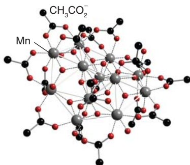
Figure 24.73* The core of the single-molecule magnetic compound \text{Mn}_{12}\text{O}_{12}(\text{O}_2\text{CMe})_{16}(\text{H}_2\text{O})_4 \cdot 2\text{MeCO}_2\text{H} \cdot 4\text{H}_2\text{O} that contains 12 Mn(III) and Mn(IV) centres.
