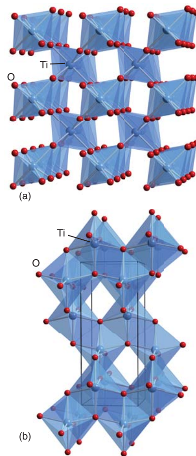
Figure 24.66 \text{TiO}_2 exists as several polymorphs that can be described in terms of linked \text{TiO}_6 octahedra, including the (a)* rutile and (b)* anatase forms.
