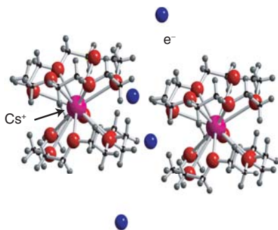
Figure 11.15* The crystal structure of [\text{Cs}(18\text{-crown-6})]_2^+e^- . The blue spheres mark the sites of highest electron density and so indicate the locations of the 'anion' e^- .
