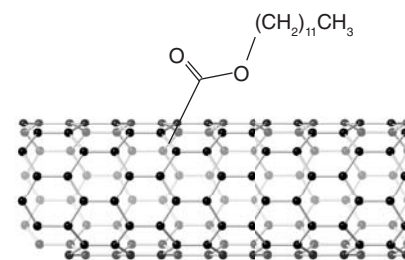
Figure 24.94 Ester-functionalized SWNT (SWNT-COO(CH 2 ) 11 CH 3 ). (Based on R. Sen, et al., Nano Lett. , 2004, 4, 459.)
