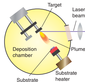
Figure 24.78 A pulsed laser deposition chamber used to produce nanostructured super lattices and artificially layered thin films.
