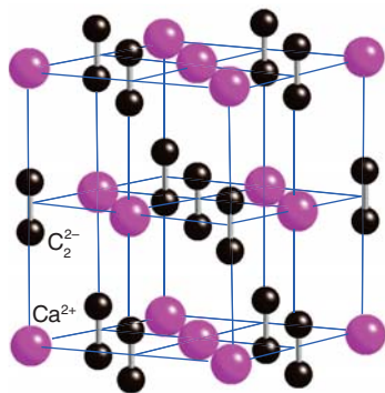
Figure 3.31* The structure of \text{CaC}_2 is based on the rock-salt structure but is elongated in the direction parallel to the axes of the \text{C}_2^{2-} ions.
