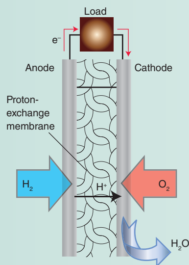
Figure B5.1 A schematic diagram of a proton-exchange membrane (PEM) fuel cell. The anode and cathode are loaded with a catalyst (Pt) to convert fuel ( \text{H}_2 ) and oxidant ( \text{O}_2 ) into \text{H}^+ and \text{H}_2\text{O} respectively. The membrane (usually a material called Nafion ^{\text{®}} ) allows the \text{H}^+ ions produced at the anode to be transferred to the cathode.
