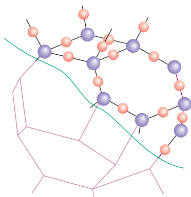
Figure 14.19 Framework representation of a truncated octahedron (truncation perpendicular to the fourfold axes of the octahedron) and the relationship of Si and O atoms to the framework. Note that a Si atom is at each vertex of the truncated octahedron and an O atom is approximately along each edge.
