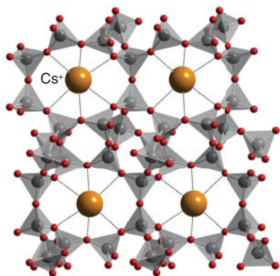
Figure 24.49* The clinoptililite structure, highlighting the relationship between the trapped \text{Cs}^+ ions, shown as spheres with ionic radius 180 pm, and the framework.
