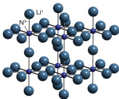
Figure 11.11* The structure of \text{Li}_3\text{N} .
