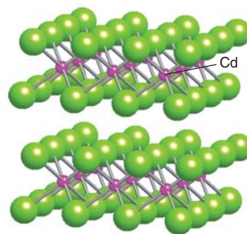
Figure 16.3 The CdI_2 structure adopted by many disulfides.
