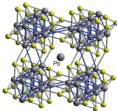
Figure 24.44* The structure of a Chevrel phase showing the canted \text{Mo}_6\text{S}_8 units forming a slightly distorted cube around a Pb atom. An Mo atom in one cube can act as the acceptor for an electron pair donated by an S atom in a neighbouring cage.
