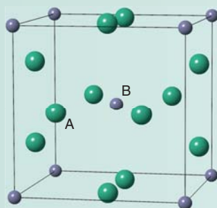
Figure B3.3 The structure of the A15 intermetallic phases.
