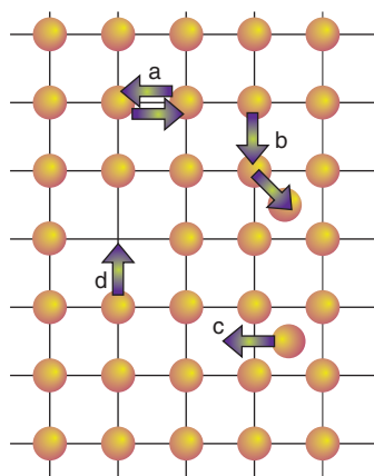
Figure 24.4 Some diffusion mechanisms for ions or atoms in a solid: (a) two atoms or ions exchange positions; (b) an ion hops from a normally occupied site in the structure to an interstitial site, which produces a vacancy which can then be filled by movement of an ion from another site; (c) an ion hops between two different interstitial sites; (d) an ion or atom moves from a normally occupied site to a vacancy, so producing a new vacant site.
