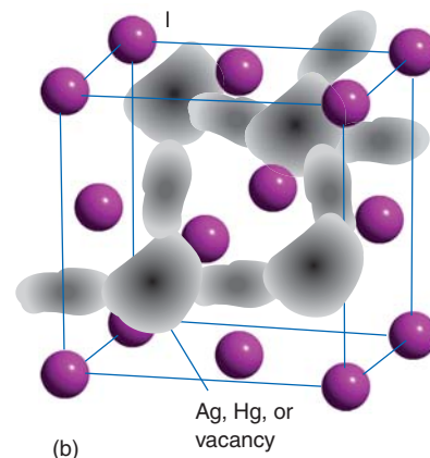
Figure 24.6* (a) Low-temperature ordered structure of \text{Ag}_2\text{HgI}_4 . (b) High-temperature disordered structure showing the cation disorder. \text{Ag}_2\text{HgI}_4 is an \text{Ag}^+ ion conductor in the high-temperature form.
