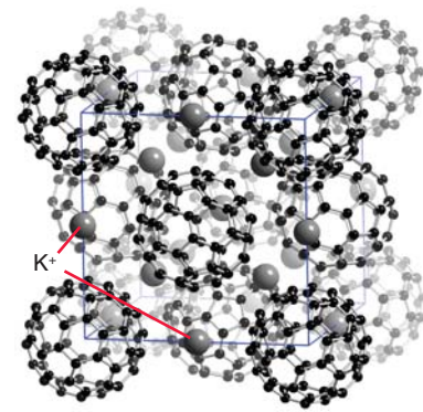
Figure 24.70* The structure of K_3C_{60} is obtained by filling all the tetrahedral and all the octahedral holes in the close-packed C_{60}^{3-} lattice with K^+ ions.
