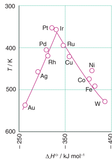
Figure 25.17 A ‘volcano diagram’, in this case the reaction temperature for a set rate of methanoic (formic) acid decomposition plotted against the stability of the corresponding metal methanoate as judged by its enthalpy of formation. (Based on W.J.M. Rootsart and W.M.H. Sachtler, Z. Physik. Chem. 1960, 26 , 16.).
