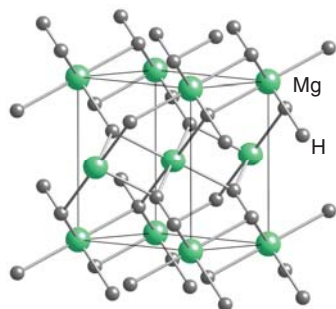
Figure 24.59* The structure of MgH_2 .
