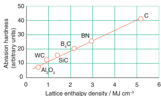
Figure 13.6 The correlation of hardness with lattice enthalpy density (the lattice enthalpy divided by the molar volume of the substance). The point for carbon represents diamond; that for boron nitride represents the diamond-like sphalerite structure.
