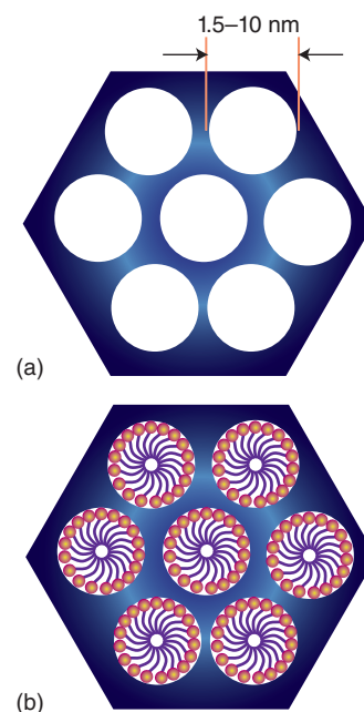
Figure 24.89 A hexagonal mesoporous structure with (a) controlled nanoporosity and (b) functionalized pores.
