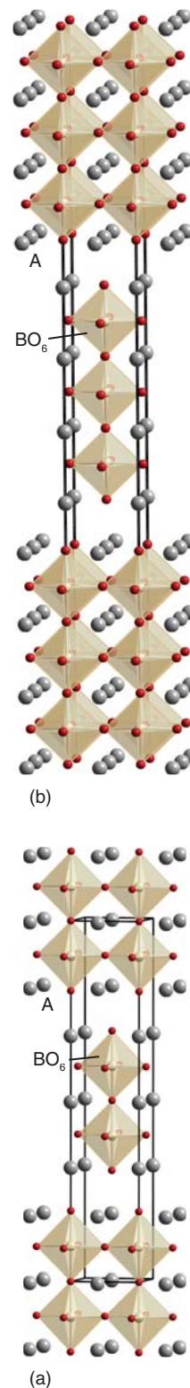
Figure 24.22* The Ruddlesden–Popper phases of stoichiometry (a) \text{A}_3\text{B}_2\text{O}_7 and (b) \text{A}_4\text{B}_3\text{O}_{10} , formed respectively from two and three perovskite layers of linked \text{BO}_6 octahedra separated by A-type cations.
