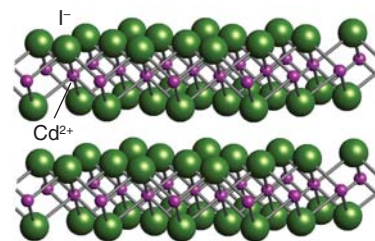
Figure 3.40* The \text{CdI}_2 structure.
