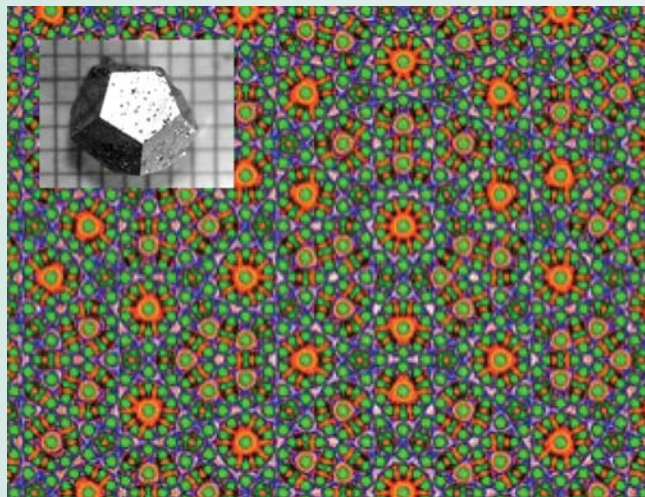
Figure B3.2 Computer-generated representation of a quasi-crystal showing five-fold symmetry. Inset, a photograph of a dodecahedral quasicrystal.
