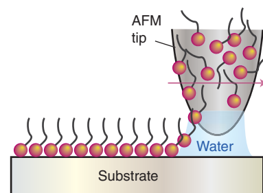
Figure 24.79 The process of dip-pen nanolithography. Organothiols move from an AFM tip through a water meniscus, forming a self-assembled monolayer on a gold substrate. (Adapted from C. Mirkin, Nanoscience Boot Camp at Northwestern University 2001.)
