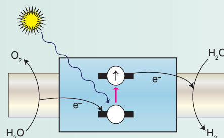
Figure B10.3 The principle of a water-splitting device for solar \text{H}_2 generation: visible light excites an electron into an upper energy level (conduction band); the 'hot' electron is delivered to the catalyst that converts \text{H}^+ (from \text{H}_2\text{O} ) into \text{H}_2 ; the 'hole' in the lower level (valence band) is filled by an electron delivered from the catalyst that converts \text{H}_2\text{O} to \text{O}_2 . In order to convey the principle in the simplest terms, the associated oxidation and reduction reactions in the text have not been balanced.
