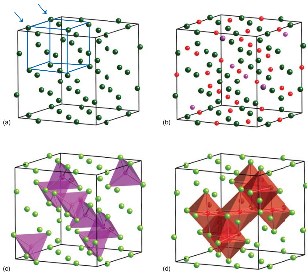
Figure 3.44 The spinel structure AB_2O_4 : (a) the close-packed arrangement of anions ( O^{2-} ) in the full unit cell (close-packed layers are arrowed); the smaller simple ccp unit cell is outlined in blue; (b) the arrangement of cations and anions within the full unit cell with the A cations shown in magenta and B cations in red; (c)* and (d) the polyhedral coordination of A (tetrahedral) and B (octahedral) by oxide for cation sites fully within the unit cell.
