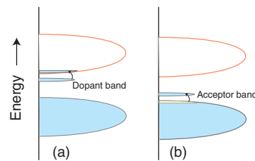
Figure 3.73 The band structure in (a) an n-type semiconductor and (b) a p-type semiconductor.
