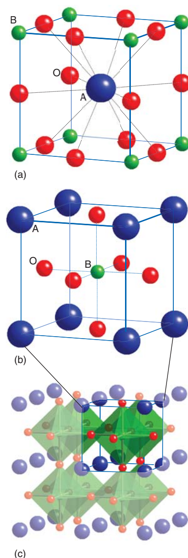
Figure 24.19* Views of the perovskite (ABO 3 ) structure (a) emphasizing the 12-fold coordination of the larger A cation and showing the relationship with the ReO 3 structure of Fig. 23.22b, (b) highlighting the octahedral coordination of the B cation. (c) A polyhedral representation accentuating the BO 6 octahedra.
