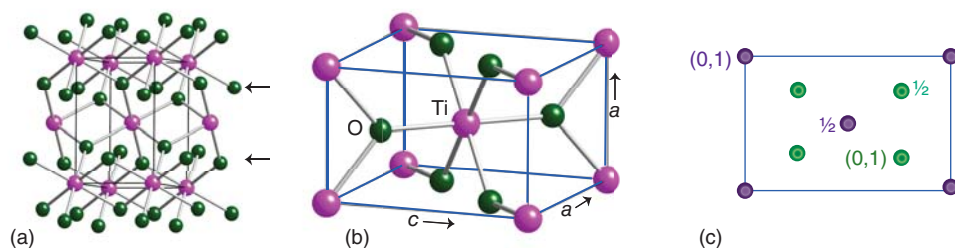
Figure 3.39 The rutile structure adopted by one polymorph of \text{TiO}_2 : (a) the buckled close-packed layers of oxide ions with titanium cations in half the octahedral holes (the unit cell is outlined); (b)* the unit cell, showing the titanium coordination to oxide ions; and (c) its projection representation.
