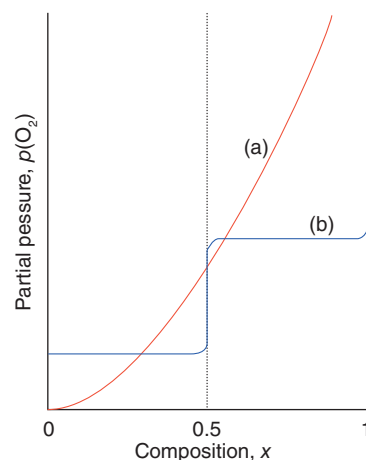
Figure 3.58 Schematic representation of the variation of the partial pressure of oxygen with composition at constant pressure for (a) a nonstoichiometric oxide \text{MO}_{1+x} and (b) a stoichiometric pair of metal oxides \text{MO} and \text{MO}_2 . The x -axis is the atom ratio in \text{MO}_{1+x} .
