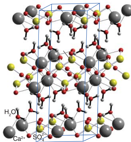
Figure 12.8 The structure of \text{CaSO}_4 \cdot 2\text{H}_2\text{O} , highlighting the water molecules that are mainly lost on heating above 150^\circ\text{C} .
