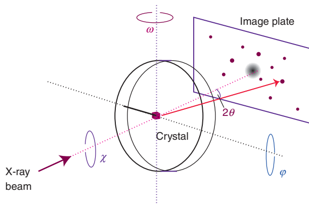
Figure 8.5 The layout of a four-circle diffractometer. A computer controls the location of the detector as the four angles are changed systematically.
