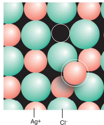
Figure 3.54 A Frenkel defect forms when an ion moves to an interstitial site.
