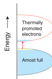
Figure 3.72 In an intrinsic semiconductor, the band gap is so small that the Fermi distribution results in the population of some orbitals in the upper band.
