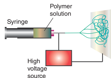
Figure 24.93 The electrospinning apparatus. (Adapted from R. Sen, et al., Nano Lett. , 2004, 4, 459.)
