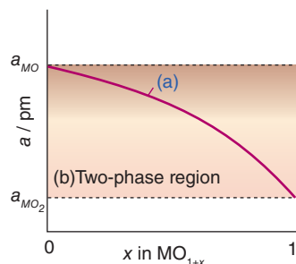
Figure 3.59 Schematic representation of the variation of one lattice parameter with composition for (a) a nonstoichiometric oxide \text{MO}_{1+x} and (b) a stoichiometric pair of metal oxides \text{MO} and \text{MO}_2 with no intermediate stoichiometric phases (which would produce a two-phase mixture for 0 < x < 1 , each phase in the mixture having the lattice parameter of the end member).
