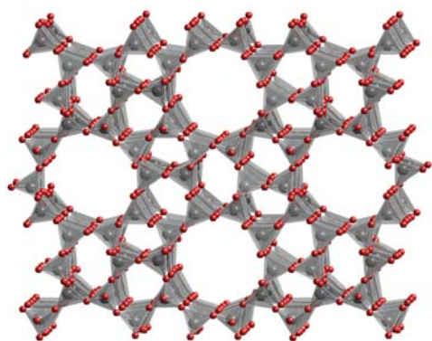
Figure 25.23* The zeolite ZSM-5 structure, highlighting the channels along which small molecules may diffuse. Tetrahedra are \text{SiO}_4 or \text{AlO}_4 .
