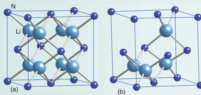
Figure B10.4 Structural relationship between (a)* Li 2 NH (antifluorite structure) and (b)* LiNH 2 (note Li vacancies), which may facilitate transport of Li + ions and reversible uptake of H 2 in conjunction with formation of a contiguous LiH phase (not shown). Hydrogen atoms are omitted for clarity.
