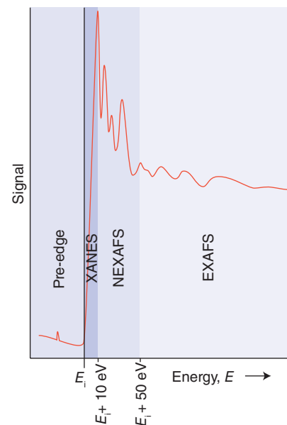
Figure 8.38 A typical X-ray absorption-edge spectrum defining the various regions discussed in the text.
