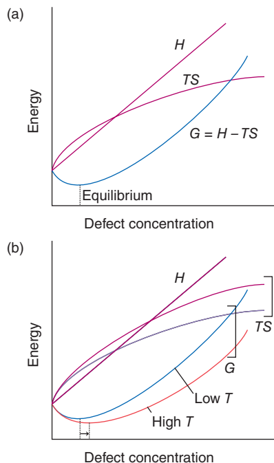
Figure 3.52 (a) The variation of the enthalpy and entropy of a crystal as the number of defects increases. The resulting Gibbs energy G = H - TS has a minimum at a nonzero concentration, and hence defect formation is spontaneous. (b) As the temperature is increased, the minimum in the Gibbs energy moves to higher defect concentrations, so more defects are present at equilibrium at higher temperatures than at low temperatures.
