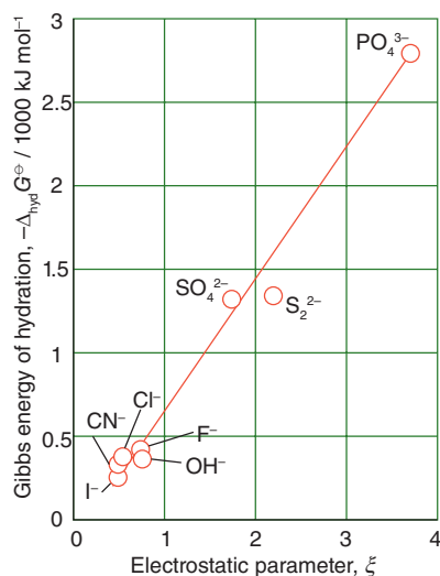
Figure 4.3 The correlation between \Delta_{\text{solv}} G^\ominus and the dimensionless electrostatic parameter \xi (= 100z^2/(r/\text{pm})) of selected anions.
