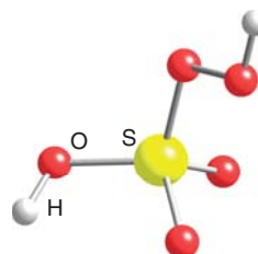
30 Peroxomonosulfuric acid, \text{H}_2\text{SO}_5
