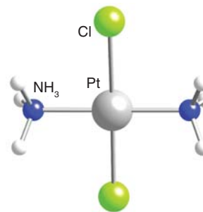
39 trans - [\text{PtCl}_2(\text{NH}_3)_2]
