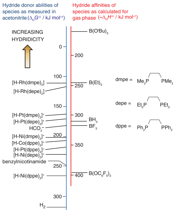
Figure 10.15 Scaling hydridicity: the right-hand scale shows values of hydride affinities ( -\Delta_{\text{H}}H^\ominus ) calculated for some boron compounds using density functional theory; the left-hand scale shows hydride-donor abilities ( \Delta_{\text{H}}G^\ominus ) for bis(diphosphine) d-metal complexes and other species, calculated from experimental data obtained in solution. The two scales are aligned using the observed equilibrium constant of approximately 1 between [\text{HRh}(\text{dmpe})_2] and \text{BET}_3 . (Figure adapted from Mock et al., J. Am. Chem. Soc. , 2009, 131, 14454, and other data.)
