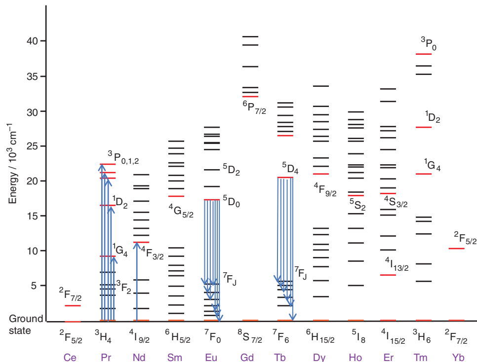
Figure 23.6 Simplified energy-level diagram for the lanthanoids. Upward arrows for \text{Pr}^{3+} and \text{Nd}^{3+} represent principal absorption lines for those ions. Downward arrows for \text{Eu}^{3+} and \text{Tb}^{3+} represent the principal emission lines for those ions.
