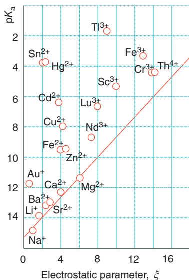
Figure 4.4 The correlation between acidity constant pK_a and the dimensionless electrostatic parameter \xi (= 100z^2/(r/\text{pm})) of aqua ions.
