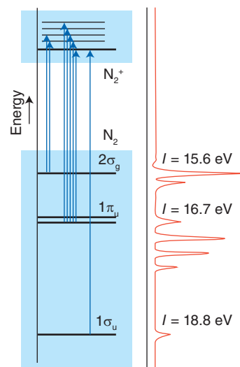
Figure 2.11 The UV photoelectron spectrum of \text{N}_2 . The fine structure in the spectrum arises from excitation of vibrations in the cation formed by photoejection of an electron.
