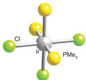
71 mer - [\text{IrCl}_3(\text{PMe}_3)_3]
