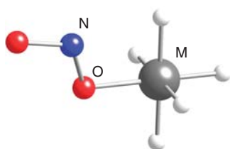
5 Nitrito- \kappa\text{O} ligand
