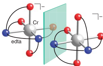
75 [\text{Cr}(\text{edta})]^- enantiomers
