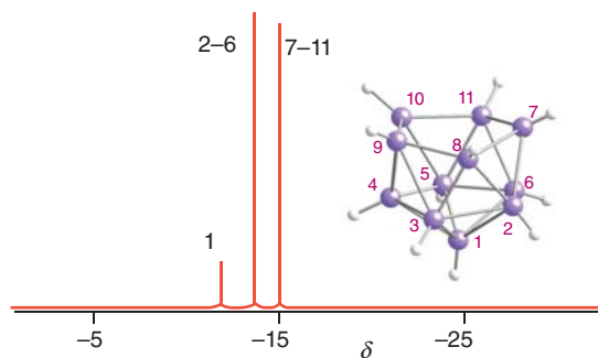
Figure 13.13 The proton-decoupled ^{11}\text{B} -NMR spectrum of [\text{B}_{11}\text{H}_{14}]^- . The nido structure (a truncated icosahedron) is indicated by the 1:5:5 pattern.
