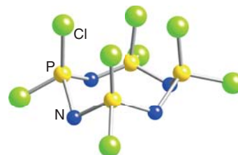
29 (\text{Cl}_2\text{PN})_4
