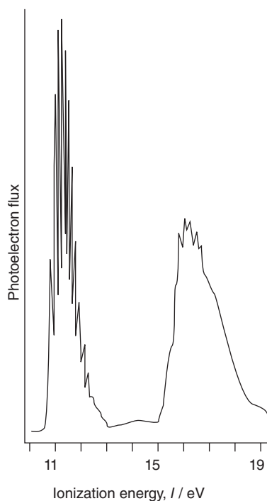
Figure 2.28 The UV photoelectron spectrum of NH_3 , obtained using He 21 eV radiation.
