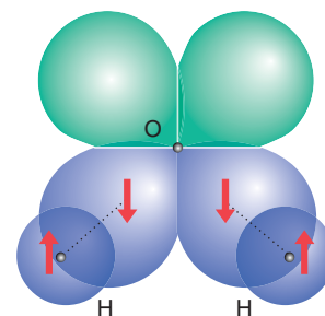
Figure 2.6 The VB description of H_2O . There are two \sigma bonds formed by pairing electrons in O2p and H1s orbitals. This model predicts a bond angle of 90^\circ .
