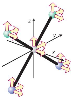
Figure 6.27* The atomic displacements in cis -[PdCl 2 (NH 3 ) 3 ] with the H atoms ignored.
