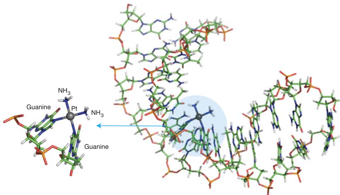
Figure 27.3 Structure of a complex formed between the Pt(NH 3 ) 2 fragment and two adjacent guanine bases on an oligonucleotide. Left: The square-planar ligand arrangement around the Pt atom. Right: Coordination of Pt causes bending of the DNA helix.
