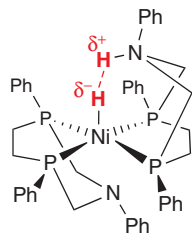
13 Functional analogue of a hydrogenase
