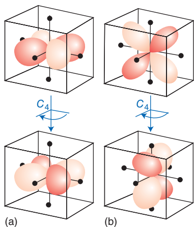
Figure 20.26* The changes in sign that occur under C_4 rotations about the z -axis: (a) a d_{xy} orbital is rotated into the negative of itself; (b) a d_{yz} orbital is rotated into a d_{zx} orbital.
