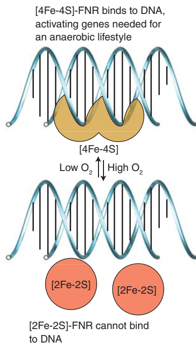
Figure 26.53 The principle of operation of the fumarate-nitrate regulatory system that controls aerobic vs anaerobic respiration in bacteria.
