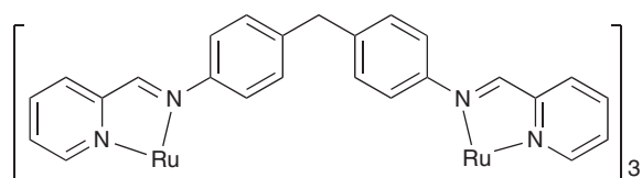
9 Ru cylinder complex
