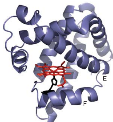
Figure 26.15* Structure of myoglobin, showing the Fe–porphyrin group located between helices E and F.
