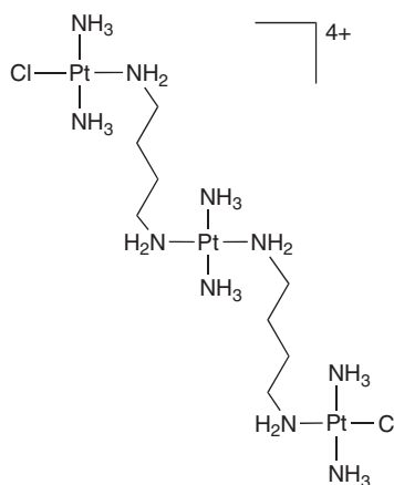
4 Trinuclear Pt(II) anticancer complex
