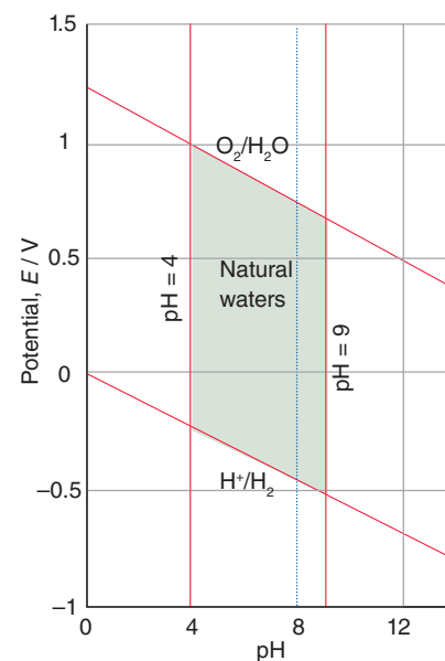
Figure 5.3 The variation of the reduction potentials of water with pH. The sloping lines defining the upper and lower limits of thermodynamic water stability are the potentials for the \text{O}_2/\text{H}_2\text{O} and \text{H}^+/\text{H}_2 couples, respectively. The central zone represents the stability range of natural waters.
