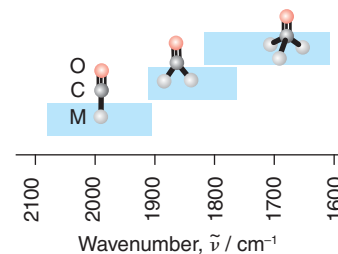
Figure 22.4 Approximate ranges for CO stretching bands in neutral metal carbonyls. Note that high wavenumbers (and hence high frequencies) are on the left, in keeping with the way infrared spectra are generally plotted.
