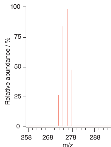
Figure 8.43 The mass spectrum of \text{ClBr}_3 .
