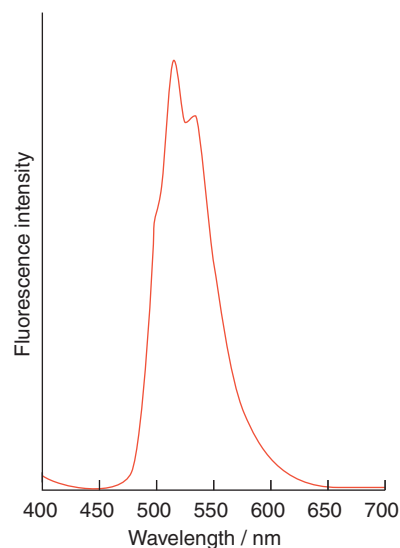
Figure 23.18 Emission spectrum of the the uranyl ion, \text{UO}_2^{2+} , excited with UV radiation.
