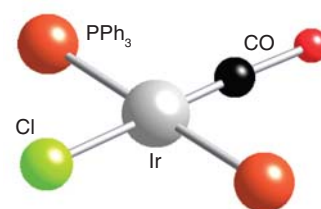
6 \text{trans-}[\text{IrCl}(\text{CO})(\text{PPh}_3)_2]
