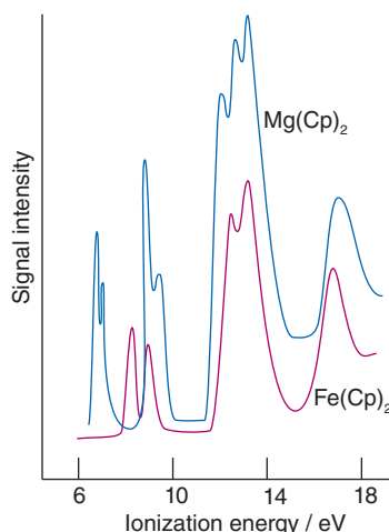
Figure 20.18 Photoelectron spectra of ferrocene and magnesocene.
