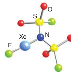
11 \text{FXeN}(\text{SO}_2\text{F})_2
