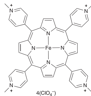
14 [\text{Fe}(\text{TMPyP})]^{4+}
