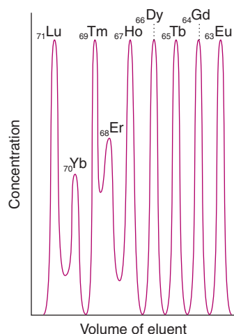
Figure 23.13 Elution of heavy Ln(III) ions from a cation-exchange column using ammonium 2-hydroxyisobutyrate as the eluent. Note that the higher atomic number lanthanoids elute first because they have smaller radii and are more strongly complexed by the eluent.
