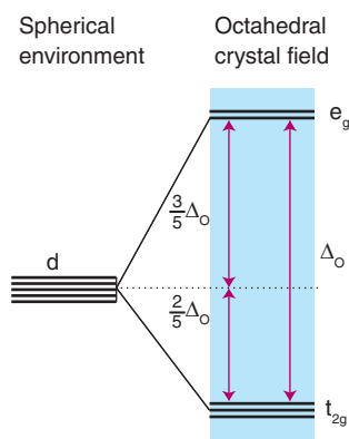
Figure 20.2 The energies of the d orbitals in an octahedral crystal field. Note that the mean energy remains unchanged relative to the energy of the d orbitals in a spherically symmetrical environment (such as in a free atom).
