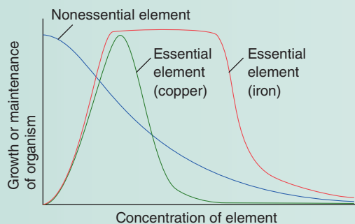
Figure B19.6 Idealized dose-response curves for a nonessential and two essential elements.
