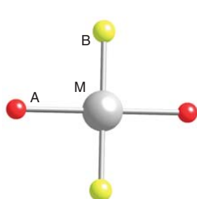
41 trans - [\text{MA}_2\text{B}_2]
