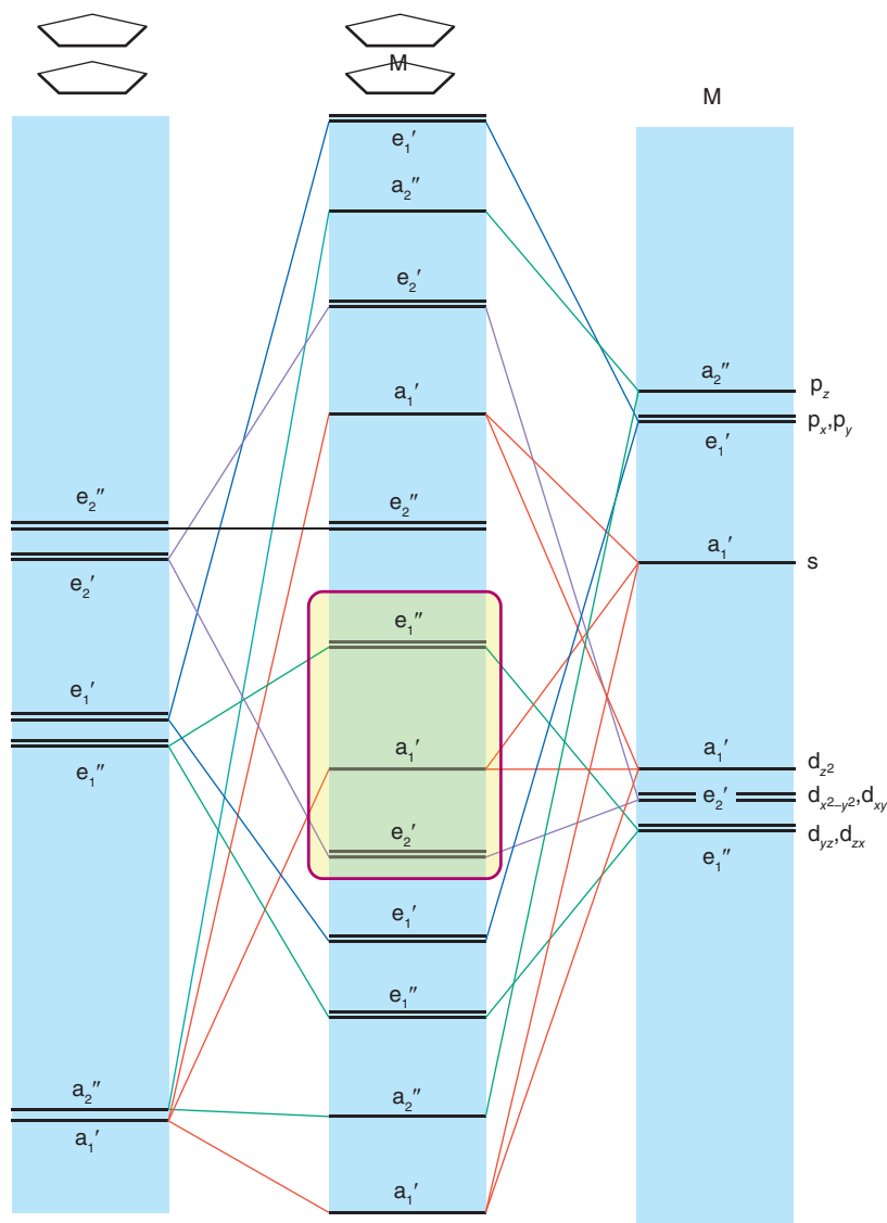
Figure 22.13 Molecular orbital energy-level diagram for a [\text{M}(\text{Cp})_2] with D_{5h} symmetry. The energies of the symmetry-adapted \pi orbitals of the \text{C}_5\text{H}_5 ligands are shown on the left, relevant d orbitals of the metal are on the right, and the resulting molecular orbital energies are in the centre. Eighteen electrons can be accommodated by filling the molecular orbitals up to and including the a_1' orbital in the box. The box denotes the orbitals typically regarded as frontier orbitals in these molecules.
