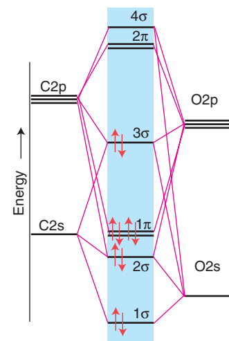
Figure 2.22* The molecular orbital energy-level diagram for CO.
