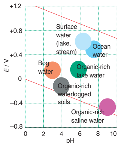
Figure 5.12 The stability field of water, showing regions typical of various natural waters.
