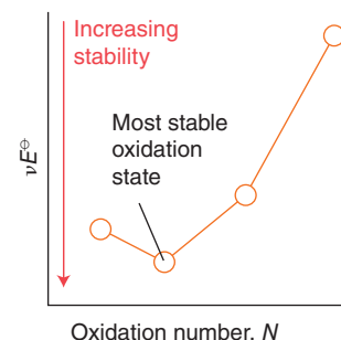
Figure 5.5 Oxidation state stability as viewed in a Frost diagram.
