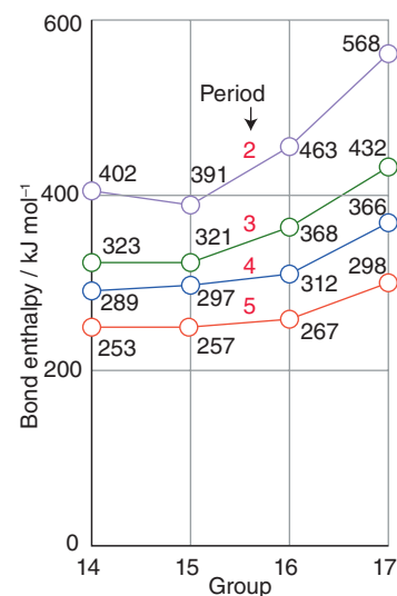
Figure 10.3 Average bond energies ( \text{kJ mol}^{-1} ) for binary molecular hydrides of p-block elements.
