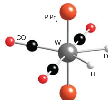
28 [\text{W}(\text{H})(\text{D})(\text{P}^i\text{Pr}_3)_2(\text{CO})_3]
