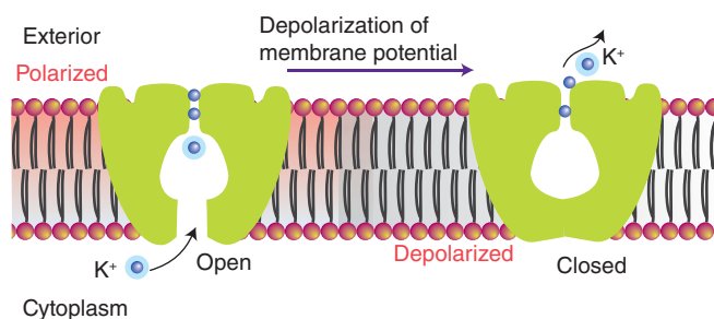
Figure 26.7 Proposed mechanism of action of the K^+ channel. The potential difference across the membrane is sensed by the protein, which causes the pore to open, allowing hydrated ions to enter the cavity. After shedding their hydration sphere, K^+ ions pass up the selectivity filter at rates close to diffusion control.
