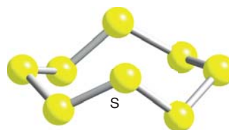
14 S_8
