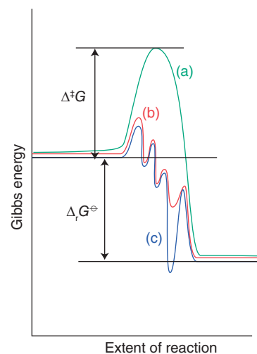
Figure 25.1 Schematic representation of the energetics of a catalytic cycle. The uncatalysed reaction (a) has a higher \Delta^\ddagger G than a step in the catalysed reaction (b). The Gibbs energy of the overall reaction, \Delta_r G^\ominus , is the same for routes (a) and (b). The curve (c) shows the profile for a reaction mechanism with an intermediate that is more stable than the product.
