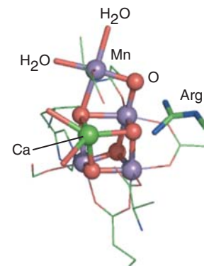
Figure 26.41 The [\text{4MnCa-5O}] active site of photosynthetic \text{O}_2 production. The Ca atom is shown in green, Mn atoms are shown in mauve, and O atoms are shown in red.
