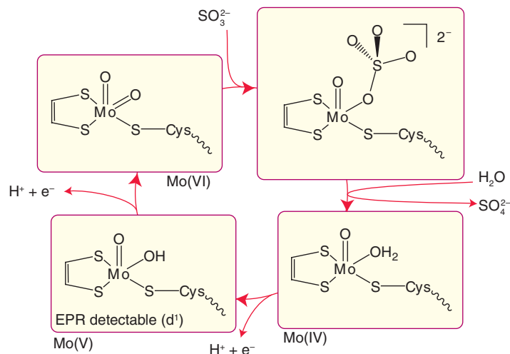
Figure 26.45 Oxidation of sulfite to sulfate by sulfite oxidase, illustrating the direct O-atom transfer mechanism for Mo enzymes.
