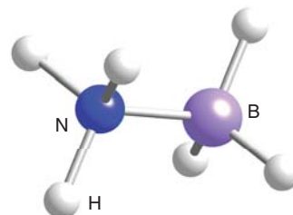
20 NH_3BH_3
