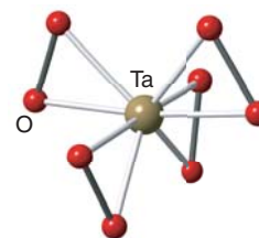
7 [Ta(\eta^2-O_2)_4]^{3-}
