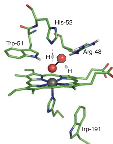
Figure 26.34* The active site of yeast cytochrome c peroxidase showing amino acids essential for activity and indicating how peroxide is bound in the distal pocket.
