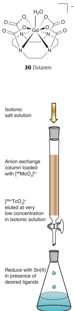
Figure 27.7 Principles of preparation of Tc-99 complexes.
