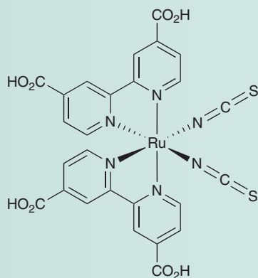
S1 cis-bis(thiocyanato- k N)bis(4,4'-dicarboxylato-2,2'-bipyridyl) ruthenium(II)
