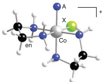
8 cis - [\text{CoAX}(\text{en})_2]^+
