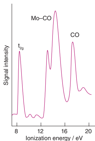
Figure 20.17 The He(II) (30.4 nm) photoelectron spectrum of [\text{Mo}(\text{CO})_6] .
