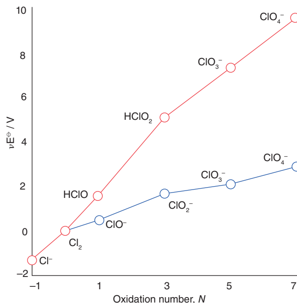
Figure 5.18 A Frost diagram for chlorine. The red line refers to acid conditions (pH=0) and the blue line to pH=14. Note that because \text{HClO}_3 and \text{HClO}_4 are strong acids, even at pH=0 they are present as their conjugate bases.
