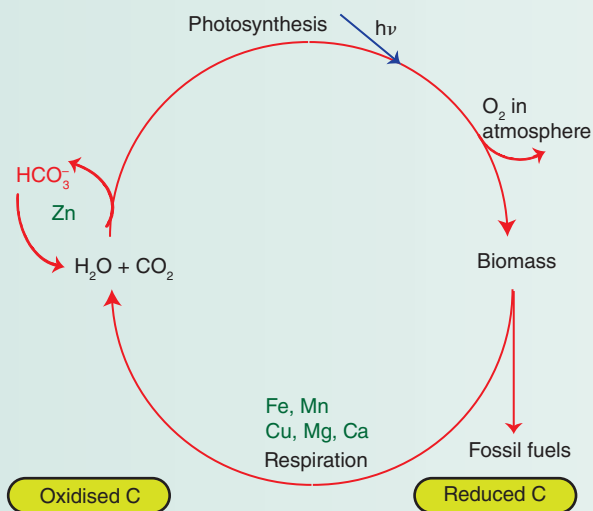
Figure B14.2 The major elements of the carbon cycle.
