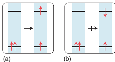
Figure 20.35 (a) A spin-allowed transition does not change the multiplicity. (b) A spin-forbidden transition results in a change in the multiplicity.
