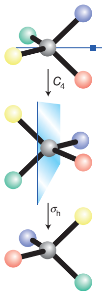
Figure 6.7* A four-fold axis of improper rotation S_4 in the CH_4 molecule. The four terminal atoms of the same element are coloured differently to help track their movement.
