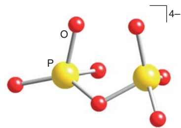
11 \text{P}_2\text{O}_7^{4-}
