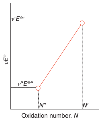
Figure 5.8 The general structure of a region of a Frost diagram used to establish the relationship between the slope of a line connecting species having different oxidation numbers and the standard potential of the corresponding redox couple.
