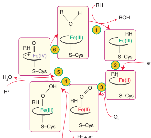
Figure 26.38 The catalytic cycle of cytochrome P450.
