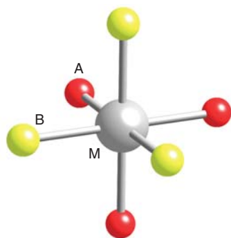
58 fac -[MA 3 B 3 ]
