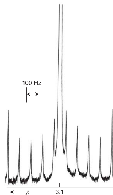
Figure 8.25 The ^1\text{H} -NMR spectrum of \text{GeH}_4 . The main resonance is at \delta = 3.1 with satellites given by J(^1\text{H}-^{73}\text{Ge}) spin-spin coupling (Section 8.5c).
