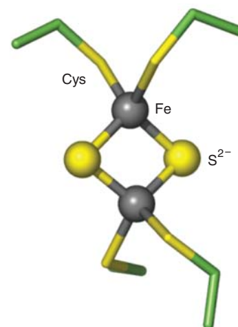
25* [2Fe-2S]
