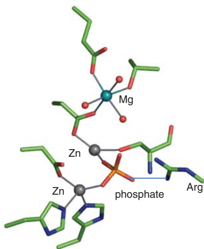
33* Active site of alkaline phosphatase
