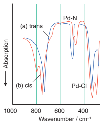
Figure 6.18 The IR spectra of cis (red) and trans (blue) forms of [\text{PdCl}_2(\text{NH}_3)_2] . (R. Layton, D.W. Sink, and J.R. Durig, J. Inorg. Nucl. Chem. , 1966, 28, 1965.)
