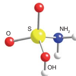
6 \text{O}_2\text{S}(\text{NH}_2)\text{OH}
