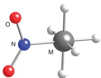
4 Nitrito- \kappa\text{N} ligand
