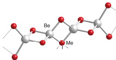
8 (\text{Be}(\text{CH}_3)_2)_n
