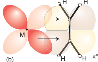
Figure 22.5* The interaction of ethene with a metal atom: (a) donation of electron density from the filled \pi molecular orbital of ethene to a vacant metal \sigma orbital; (b) acceptance of electron density from a filled d\pi orbital into the vacant \pi^* orbital of ethene.
