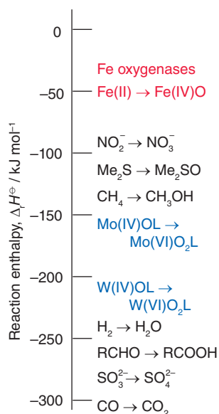
Figure 26.47 Scale showing relative enthalpies for oxygen-atom transfer. Fe(IV) oxy species are powerful O-atom donors, whereas Mo(IV) and W(IV) are good O-atom acceptors.
