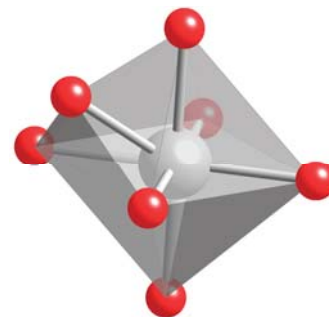
23 Capped octahedron
