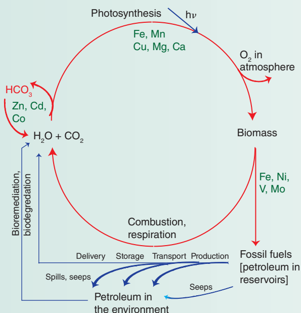
Figure B14.3 Modified carbon cycle.
