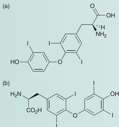
Figure B17.1 The structures of (a) thyroxine and (b) triiodothyronine.
