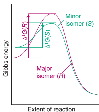
Figure 25.6 Kinetically controlled stereoselectivity. Note that \Delta^\ddagger G(S) < \Delta^\ddagger G(R) , so the minor isomer reacts faster than the major isomer.
