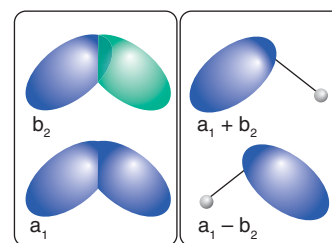
Figure 2.32 The two occupied 1a_1 and 1b_2 orbitals of the \text{H}_2\text{O} molecule and their sum 1a_1 + 1b_2 and difference 1a_1 - 1b_2 . In each case we form an almost fully localized orbital between a pair of atoms.
