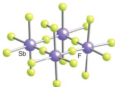
18 (\text{SbF}_5)_4
