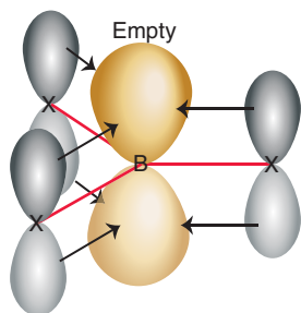
15 p–p \pi bonding in \text{BX}_3
