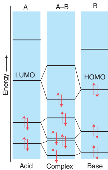
Figure 4.8 The molecular orbital representation of the orbital interactions responsible for formation of a complex between Lewis acid A and Lewis base :B.
