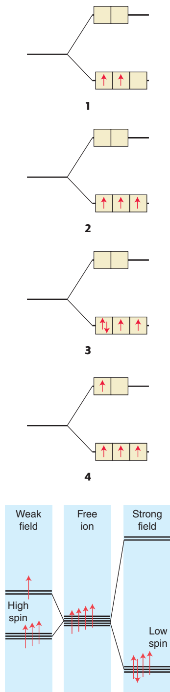
Figure 20.4 The effect of weak and strong ligand fields on the occupation of orbitals for a d^4 complex. The former results in a high-spin configuration and the latter in a low-spin configuration.
