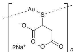
15 Myochrisin
