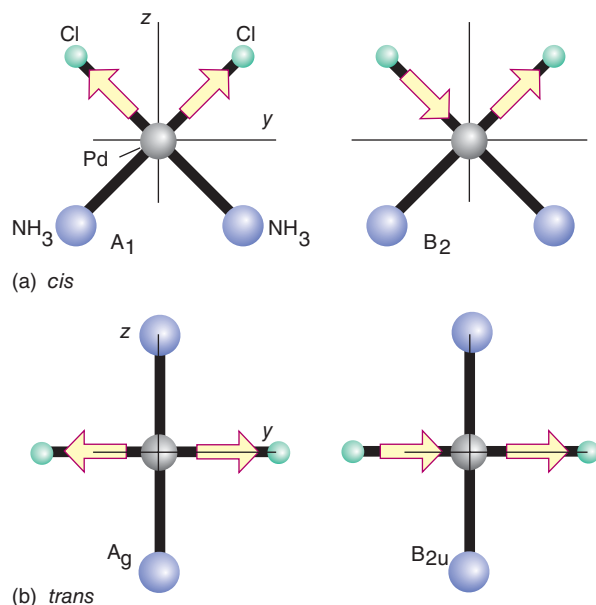
Figure 6.17* The Pd—Cl stretching modes of cis and trans forms of [\text{PdCl}_2(\text{NH}_3)_2] . The motion of the Pd atom (which preserves the centre of mass of the molecule) is not shown.
