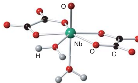
6 [Nb(OH)_2(O)(ox)_2]^-
