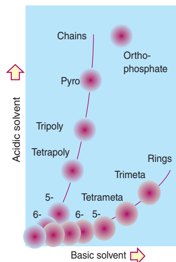
Figure 4.7 A representation of a two-dimensional paper chromatogram of a complex mixture of phosphates formed by condensation reactions. The sample spot was placed at the lower left corner. Basic solvent separation was used first, followed by acidic solvent perpendicular to the basic one. This separates open chains from rings. The upper spot sequence corresponds to linear polymers and the lower sequence corresponds to rings.
