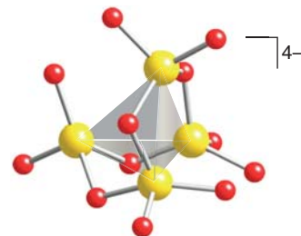
12 \text{P}_4\text{O}_{12}^{4-}
