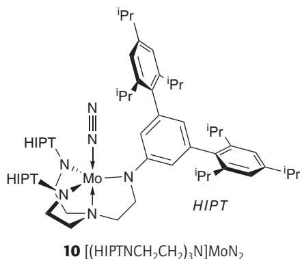
10 [(HIPTNCH_2CH_2)_3N]MoN_2
