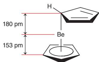
11 BeCp 2 (Cp = C 5 H 5 )
