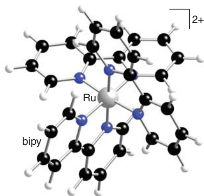
82 [\text{Ru}(\text{bpy})_3]^{2+}
