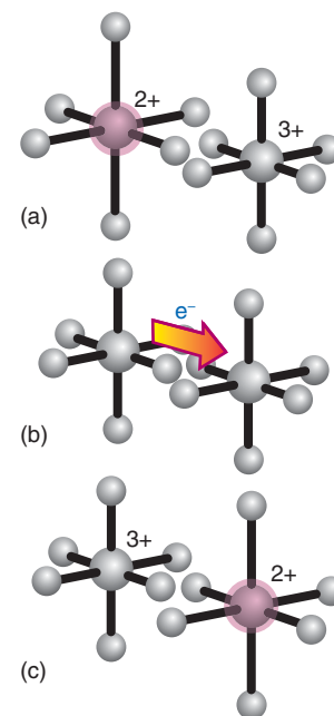
Figure 21.17* Electron transfer between two metal ions in a precursor complex is not productive until their coordination shells have reorganized to be of equal size: (a) reactants, (b) reactant complexes having distorted into the same geometry, (c) products.
