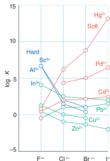
Figure 4.11 The trends in stability constants for complex formation with a variety of halide ion bases. Hard ions are indicated by blue lines, soft ions by red lines. Borderline hard or borderline soft ions are indicated by green lines.
