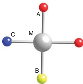
42 cis - [\text{MA}_2\text{BC}]
