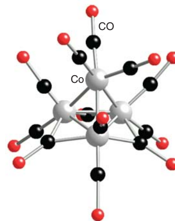
82 [\text{Co}_4(\text{CO})_{12}]
