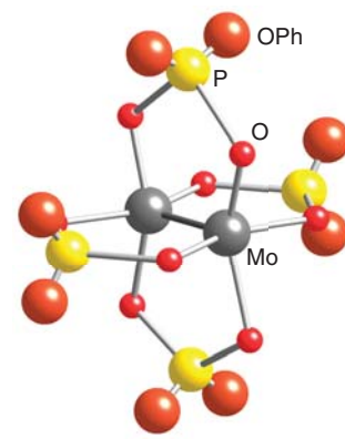
22 [\text{Mo}_2(\text{O}_2\text{P}(\text{OPh})_2)_4]
