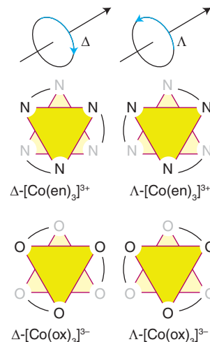
Figure 7.7* Absolute configurations of \text{M}(\text{L-L})_3 complexes. \Delta is used to indicate clockwise rotation of the helix and \Lambda to indicate anticlockwise rotation.
