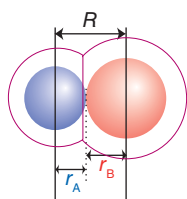
19 Covalent radius
