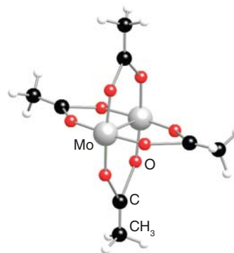
11 [\text{Mo}_2(\mu\text{-CO}_2\text{CH}_3)_4]
