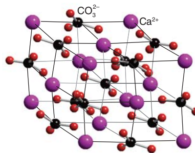
Figure 3.76* The structure of \text{CaCO}_3 .
