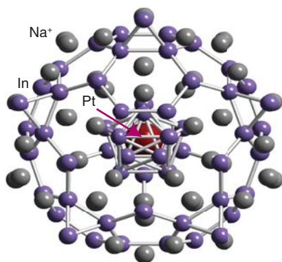
Figure 11.13* Part of the structure of \text{Na}_{172}\text{In}_{192}\text{Pt}_2 showing the complex fulleride-like networks formed by the In atoms around Na ions.
