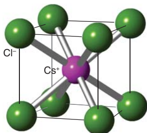
Figure 3.7* The cubic CsCl structure.
