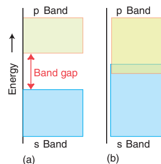
Figure 3.65 (a) The s and p bands of a solid and the gap between them. Whether or not there is in fact a gap depends on the separation of the s and p orbitals of the atoms and the strength of the interaction between them in the solid. (b) If the interaction is strong, the bands are wide and may overlap.
