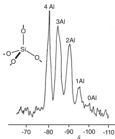
Figure 8.28 An example of a ^{29}\text{Si} -MAS-NMR spectrum obtained from the aluminosilicate zeolite analcine; each resonance represents a different silicon environment in the zeolite structure \text{Si}(\text{-OAl})_{4-n}(\text{-OSi})_n as n varies from 0 to 4.
