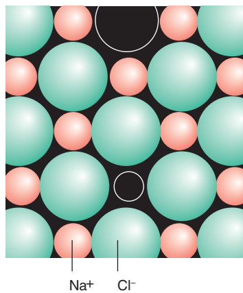
Figure 3.53 A Schottky defect is the absence of ions on normally occupied sites; for charge neutrality there must be equal numbers of cation and anion vacancies in a 1:1 compound.
