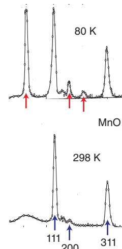
Figure 8.8 Powder neutron diffraction patterns collected from MnO showing the additional magnetic reflections that derive from the ordered antiferromagnetic arrangement of electron spins that occurs at low temperature, 80 K. MnO is paramagnetic at room temperature, with no long-range ordering of magnetic moments, so no magnetic reflection is seen at 298 K.
