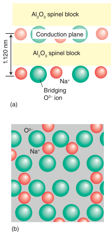
Figure 24.7 (a) Schematic side view of \beta -alumina, showing the \text{Na}_2\text{O} conduction planes between \text{Al}_2\text{O}_3 slabs. The O atoms in these planes bridge the two slabs. (b) A view of the conduction plane; note the abundance of mobile ions and vacancies in which they can move.
