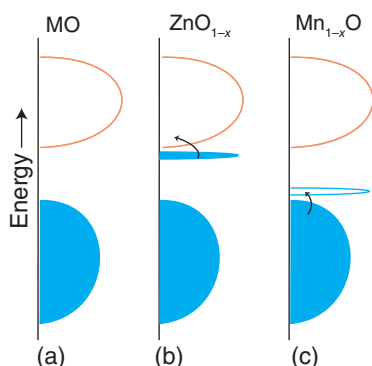
Figure 3.74 The band structure in (a) a stoichiometric oxide, (b) an anion-deficient oxide, and (c) an anion-excess oxide.
