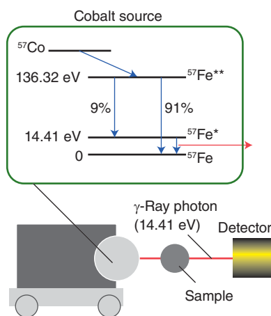
Figure 8.34 The layout of a Mössbauer spectrometer. The speed of the carriage is adjusted until the Doppler-shifted frequency of the emitted \gamma -ray matches the corresponding nuclear transition in the sample. The inset shows the nuclear transitions responsible for the emission of the \gamma -ray.
