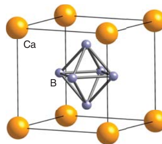
Figure 13.8 The \text{CaB}_6 structure. Note that the \text{B}_6 octahedra are connected by a bond between vertices of adjacent \text{B}_6 octahedra. The crystal is a simple cube analogue of CsCl. Thus eight Ca atoms surround the central \text{B}_6 octahedron.
