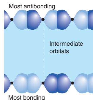
Figure 3.64 An example of a p band in a one-dimensional solid.
