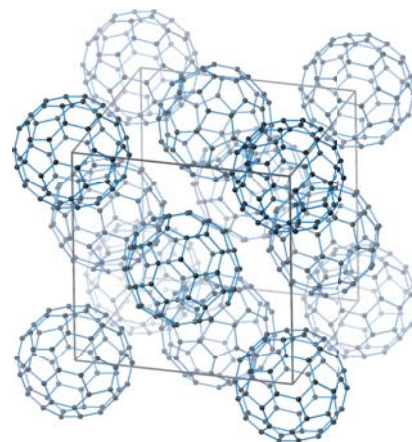
Figure 3.16* The structure of solid C 60 showing the packing of C 60 polyhedra in an fcc unit cell.
