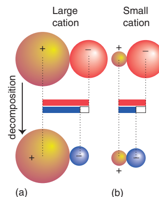
Figure 3.50 A greatly exaggerated representation of the change in lattice parameter d for cations of different radii. (a) When the anion changes size (as when CO 3 2- decomposes into O 2- and CO 2 , for instance) and the cation is large, the lattice parameter changes by a relatively small amount. (b) If the cation is small, however, the relative change in lattice parameter is large, resulting in a larger increase in lattice enthalpy, and decomposition is thermodynamically more favourable.
