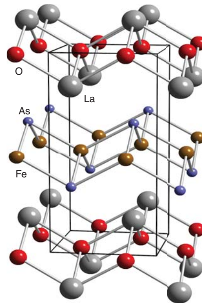
Figure 24.27* The structure of the superconductor LaFeAsO , delineating the two types of layer.
