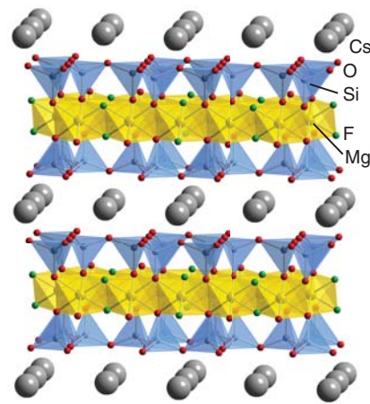
Figure 24.52* Sheet-like structures of the clay hectorite, which consist of layers of linked octahedra and tetrahedra centred on, typically, Al, Si, or Mg and separated by cations such as \text{K}^+ or \text{Cs}^+ .
