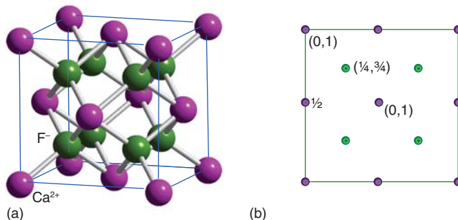
Figure 3.38 (a)* The fluorite structure and (b) its projection representation. This structure has a ccp array of cations and all the tetrahedral holes are occupied by anions.
