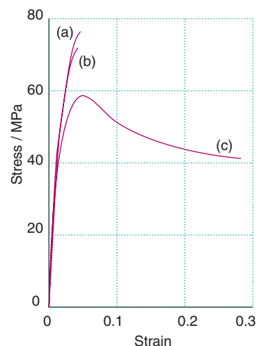
Figure 24.95 Typical stress-strain curves for (a) neat PMMA, (b) 2 per cent by mass as-received micrometre-sized alumina-filled PMMA composite, and (c) 2.2 per cent by mass 38 nm (MAA) alumina/PMMA nanocomposite. Although the strength decreases slightly for (c) (related to the decreased stress at the curve maximum), the overall ductility (related to the total strain) and toughness (related to the area under the curve) are greatly improved. (Adapted from B.J. Ash, et al., Macromolecules , 2004, 37, 1358; reproduced with permission from the American Chemical Society.)
