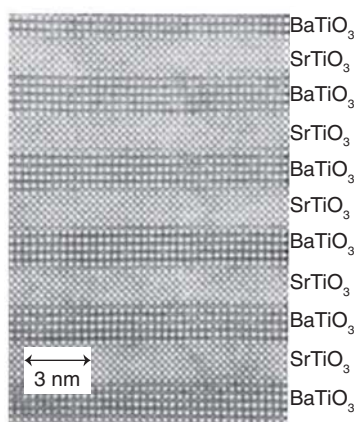
Figure 24.87 TEM image of a \text{SrTiO}_3/\text{BaTiO}_3 superlattice. (From D. G. Schlom, et al., Oxide nano-engineering using MBE. Mater. Sci. Eng. B , 2001, 87 , 282; reprinted with permission from Elsevier.)
