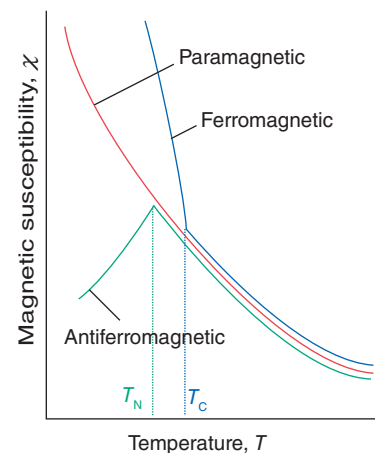
Figure 20.38 The temperature dependence of the susceptibilities of paramagnetic, ferromagnetic, and antiferromagnetic substances.
