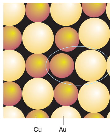
Figure 3.55 Atom exchange can also give rise to a point defect as in \text{CuAu} .
