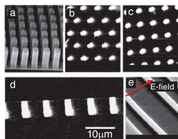
Figure 24.81 Ordered carbon nanotube structures obtained by direct chemical vapour deposition synthesis. (a) An SEM image of self-oriented MWNT arrays. Each tower-like structure is formed by many closely packed, multiwalled nanotubes. Nanotubes in each tower are oriented perpendicular to the substrate. (b) SEM top view of a hexagonal network of SWNTs (the line-like structures) suspended on top of silicon posts (the bright dots). (c) SEM top view of a square network of suspended SWNTs. (d) Side view of a suspended SWNT power line on silicon posts (the bright lines). (e) SWNTs suspended by silicon structures (the bright regions). The nanotubes are aligned along the electric field direction. (H. Dai, Acc. Chem. Res. , 2002, 35 , 1035; reproduced with permission from the American Chemical Society.).
