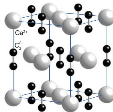
Figure 14.15* The calcium-carbide structure. Note that this structure bears a similarity to the rock-salt structure. Because \text{C}_2^{2-} is not spherical, the cell is elongated along one axis. This crystal is therefore tetragonal rather than cubic.
