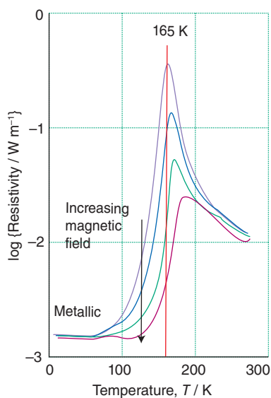
Figure 24.28 The resistivity as a function of temperature at various magnetic fields of a material displaying colossal magnetoresistance. At 165 K application of a magnetic field will cause a change in resistivity of about two orders of magnitude.
