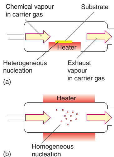
Figure 24.76 Chemical vapour methods to achieve (a) thin film growth and (b) nanoparticle production.
