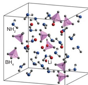
Figure 24.61* The structure of \text{Li}_3(\text{NH}_2)_2\text{BH}_4 .
