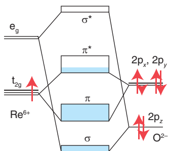
Figure 24.17 The band structure of \text{ReO}_3 .
