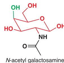
N -acetyl galactosamine
