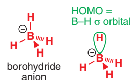
nucleophiles with a \sigma bond between electropositive atoms
