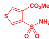
intermediate thiophene
