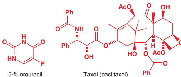
5-fluorouracil
