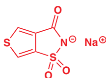
salt of thiophenesaccharin
