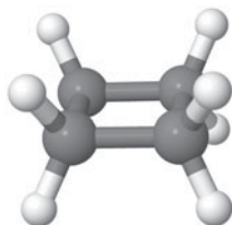
planar cyclobutane (not the real conformation)
