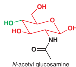
N -acetyl glucosamine
