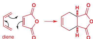
the Diels–Alder reaction
